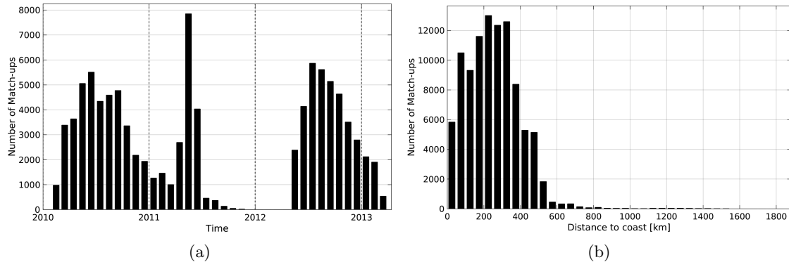
Figure 1: Number of match-ups between Surface drifters and SMOS-L3-CATDS-CECOS-LOCEAN-V2-18DAYS-25KM SSS as a function of time (a) and as function of the distance to coast (b) over the Pacific Ocean Pi-MEP region and for the full satellite product period.
