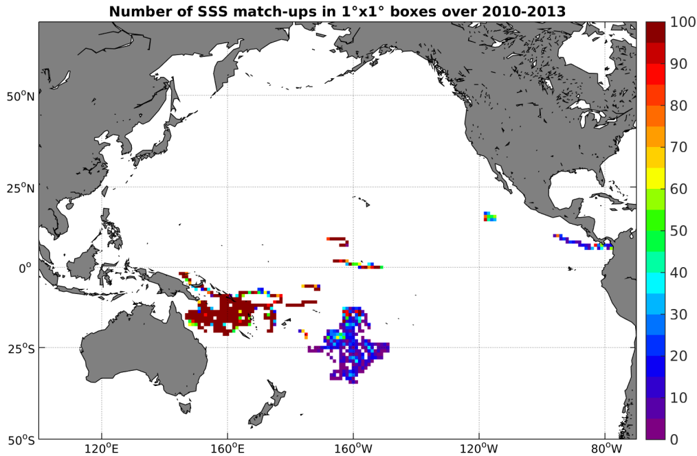
Figure 3: Number of SSS match-ups between Surface drifters SSS and the SMOS-L3-CATDS-CECOS-LOCEAN-V2-18DAYS-25KM SSS product for the Pacific Ocean Pi-MEP region over 1^\circ \times 1^\circ boxes and for the full satellite product period.
