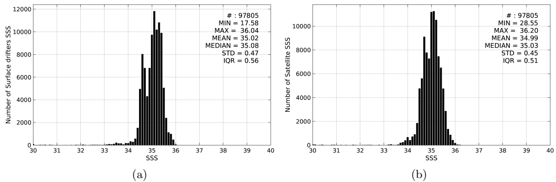
Figure 2: Histograms of SSS from Surface drifters (a) and SMOS-L3-CATDS-CECOS-LOCEAN-V2-18DAYS-25KM (b) considering all match-up pairs per bins of 0.1 over the Pacific Ocean Pi-MEP region and for the full satellite product period.
