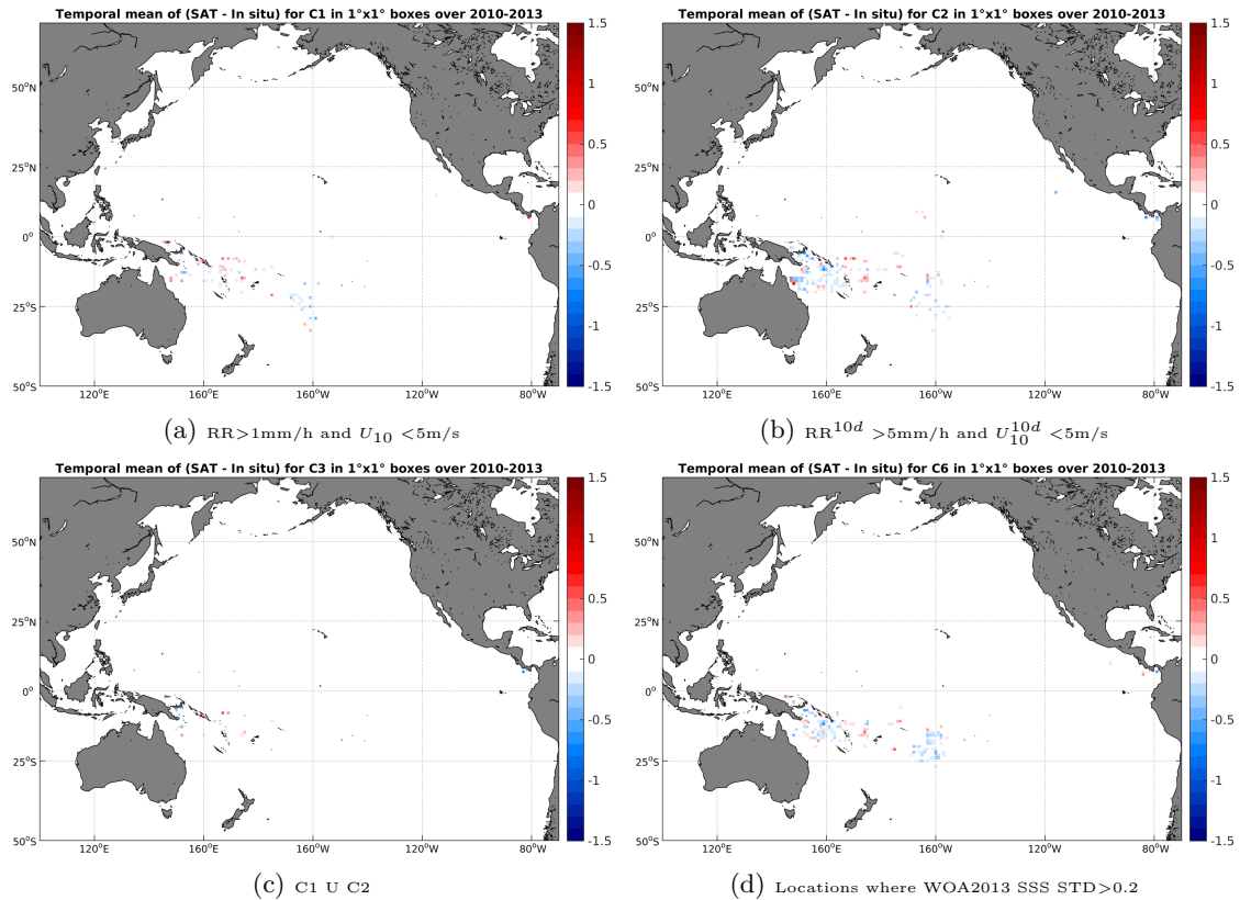
Figure 11: Temporal mean gridded over spatial boxes of size 1°x1° of \Delta SSS (SMOS-L3-CATDS-CECOS-LOCEAN-V2-18DAYS-25KM - Surface drifters) for 4 different subdatasets corresponding to:RR>1mm/h and U_{10} < 5 m/s (a), RR^{10d} > 5 mm/h and U_{10}^{10d} < 5 m/s (b), C1 U C2 (c),Locations where WOA2013 SSS STD>0.2 (d).
