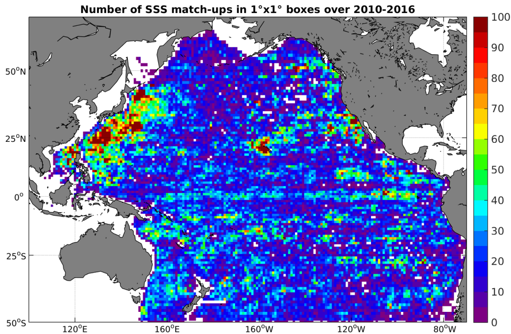
Figure 4: Number of SSS match-ups between Argo SSS and the SMOS-L3-CATDS-CECOS-LOCEAN-V2-18DAYS-25KM SSS product for the Pacific Ocean Pi-MEP region over 1^\circ \times 1^\circ boxes and for the full satellite product period.
