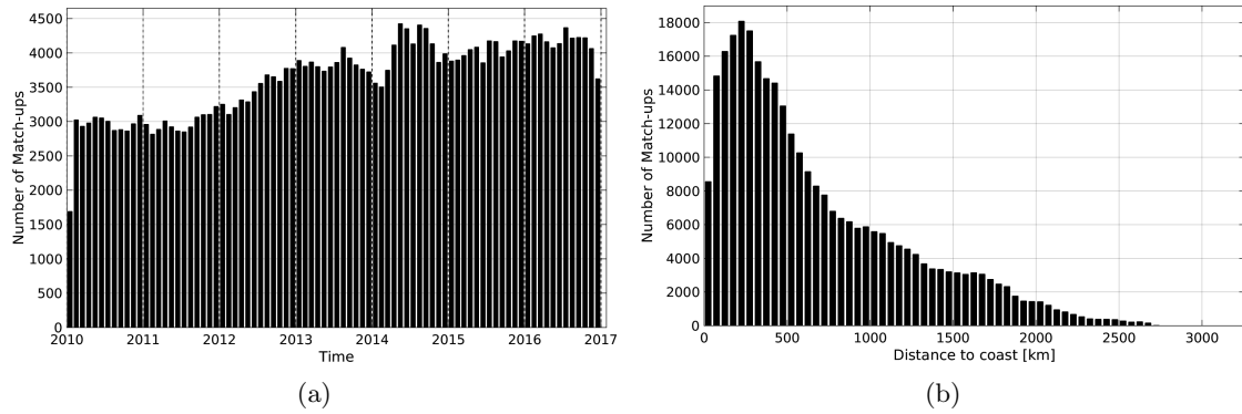
Figure 1: Number of match-ups between Argo and SMOS-L3-CATDS-CECOS-LOCEAN-V2-18DAYS-25KM SSS as a function of time (a) and as function of the distance to coast (b) over the Pacific Ocean Pi-MEP region and for the full satellite product period.
