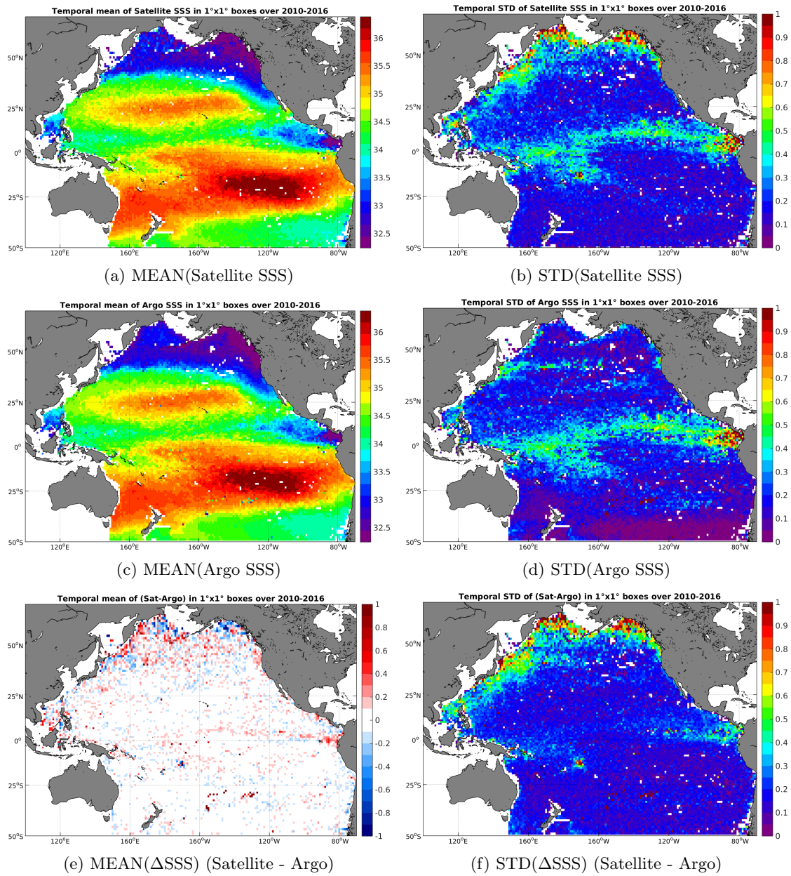
Figure 6: Temporal mean (left) and STD (right) of SSS from SMOS-L3-CATDS-CECOS-LOCEAN-V2-18DAYS-25KM (top), Argo (middle), and of \Delta SSS (Satellite - Argo). Only match-up pairs are used to generate these maps.
