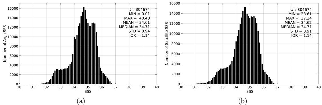
Figure 2: Histograms of SSS from Argo (a) and SMOS-L3-CATDS-CECOS-LOCEAN-V2-18DAYS-25KM (b) considering all match-up pairs per bins of 0.1 over the Pacific Ocean Pi-MEP region and for the full satellite product period.
