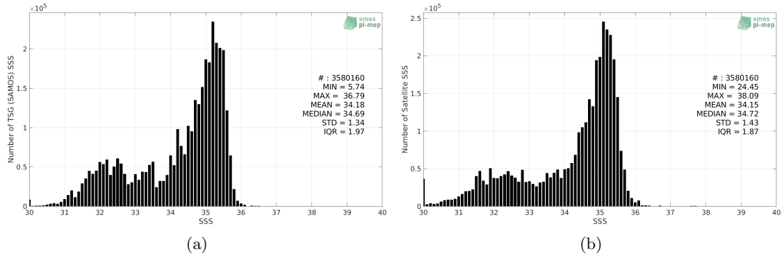
Figure 2: Histograms of SSS from TSG (SAMOS) (a) and SMOS SSS L3 v2 - Monthly - 0.25 Deg (CATDS-CECOS-IFREMER) (b) considering all match-up pairs per bins of 0.1 over the Pacific Ocean Pi-MEP region and for the full satellite product period.
