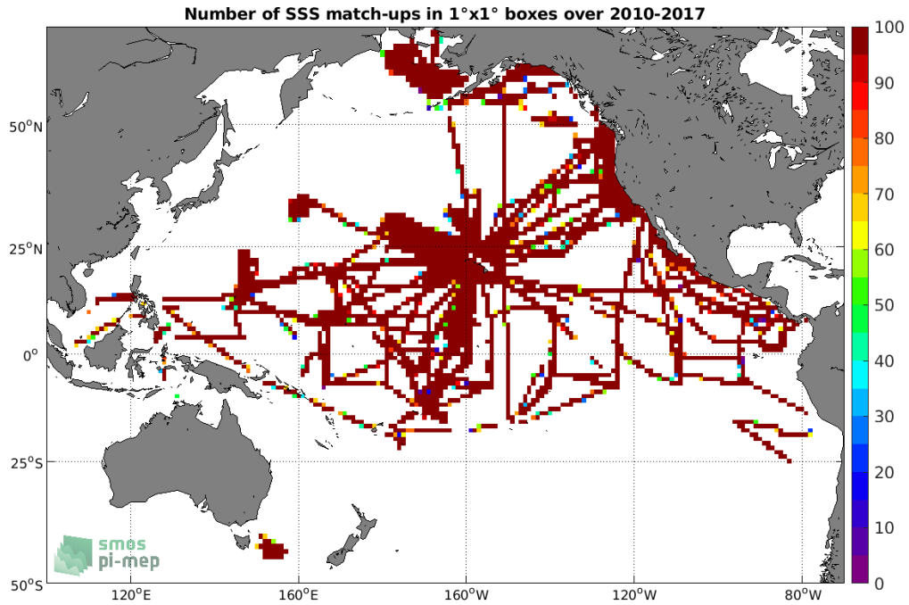
Figure 4: Number of SSS match-ups between TSG (SAMOS) SSS and the SMOS SSS L3 v2 - Monthly - 0.25 Deg (CATDS-CECOS-IFREMER) SSS product for the Pacific Ocean Pi-MEP region over 1°x1° boxes and for the full satellite product period.
