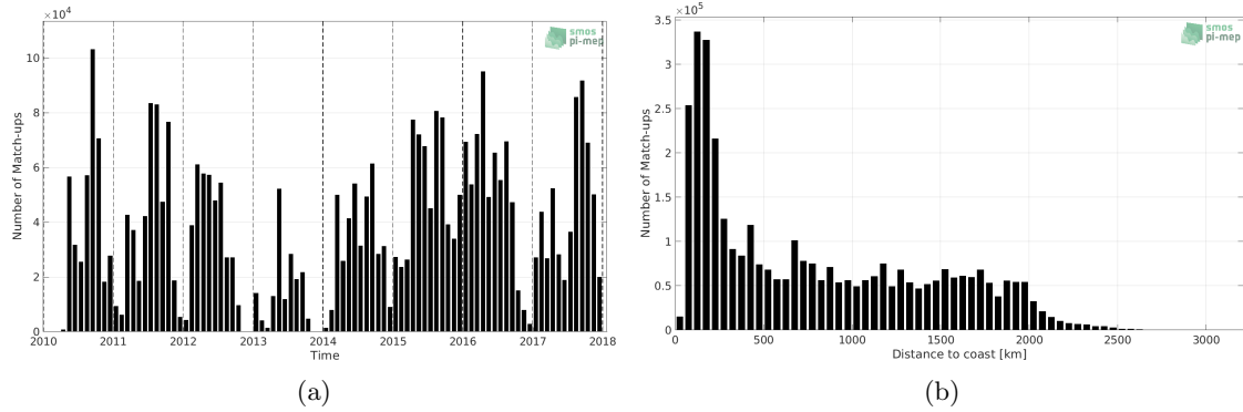
Figure 1: Number of match-ups between TSG (SAMOS) and SMOS SSS L3 v2 - Monthly - 0.25 Deg (CATDS-CECOS-IFREMER) SSS as a function of time (a) and as function of the distance to coast (b) over the Pacific Ocean Pi-MEP region and for the full satellite product period.
