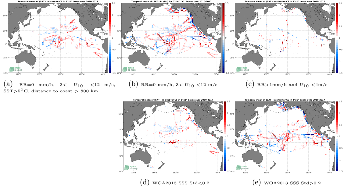
Figure 12: Temporal mean gridded over spatial boxes of size 1^\circ \times 1^\circ of \Delta SSS (SMOS SSS L3 v2 - Monthly - 0.25 Deg (CATDS-CECOS-IFREMER) - TSG (SAMOS)) for 5 different subdatasets corresponding to:RR=0 mm/h, 3 < U_{10} < 12 m/s, SST >5^\circ\text{C} , distance to coast > 800 km (a), RR=0 mm/h, 3 < U_{10} < 12 m/s (b), RR >1 mm/h and U_{10} < 4 m/s (c), WOA2013 SSS Std <0.2 (d), WOA2013 SSS Std >0.2 (e).
