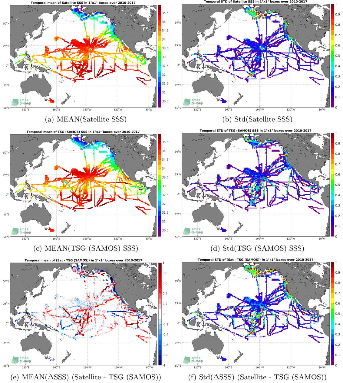
Figure 6: Temporal mean (left) and Std (right) of SSS from SMOS SSS L3 v2 - Monthly - 0.25 Deg (CATDS-CECOS-IFREMER) (top), TSG (SAMOS) (middle), and of \Delta SSS (Satellite - TSG (SAMOS)). Only match-up pairs are used to generate these maps.
