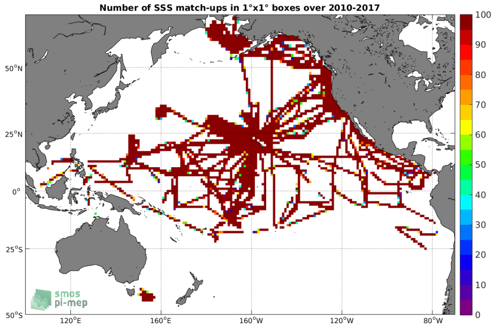
Figure 4: Number of SSS match-ups between TSG (SAMOS) SSS and the SMOS SSS L3 v2 - Monthly - 0.25 Deg (CATDS-CECOS-IFREMER) SSS product for the Pacific Ocean Pi-MEP region over 1^\circ \times 1^\circ boxes and for the full satellite product period.
