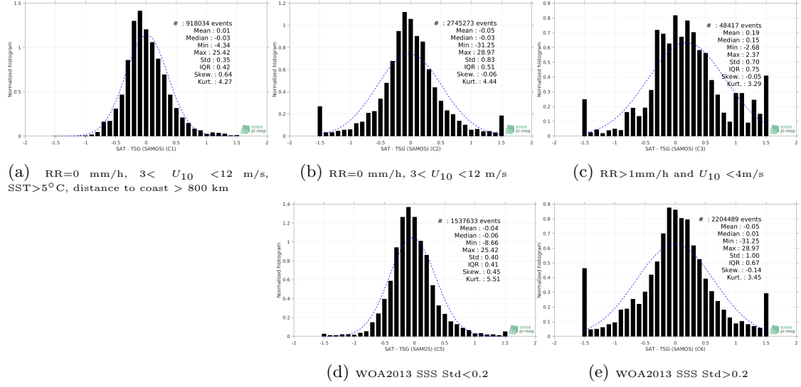
Figure 13: Normalized histogram of \Delta\text{SSS} (SMOS SSS L3 v2 - Monthly - 0.25 Deg (CATDS-CECOS-IFREMER) - TSG (SAMOS)) for 5 different subdatasets corresponding to: RR=0 mm/h, 3 < U_{10} < 12 m/s, SST > 5^\circ\text{C} , distance to coast > 800 km (a), RR=0 mm/h, 3 < U_{10} < 12 m/s (b), RR > 1 mm/h and U_{10} < 4 m/s (c), WOA2013 SSS Std < 0.2 (d), WOA2013 SSS Std > 0.2 (e).
