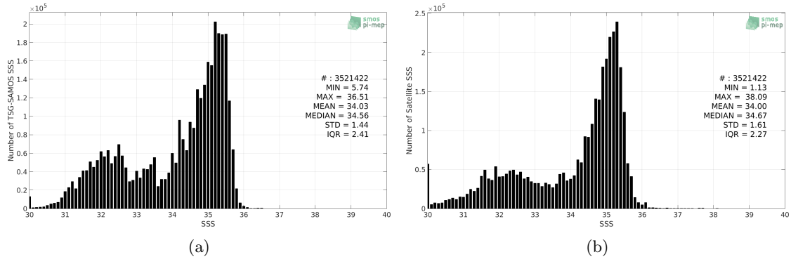
Figure 2: Histograms of SSS from TSG-SAMOS (a) and SMOS L3 v2 - Monthly - 0.25 Deg (CATDS-CECOS-IFREMER) (b) considering all match-up pairs per bins of 0.1 over the Pacific Ocean Pi-MEP region and for the full satellite product period.
