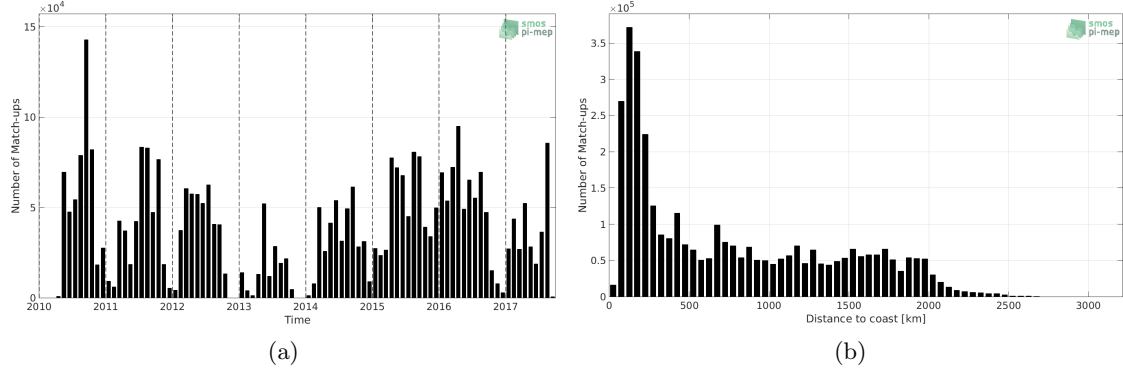
Figure 1: Number of match-ups between TSG-SAMOS and SMOS L3 v2 - Monthly - 0.25 Deg (CATDS-CECOS-IFREMER) SSS as a function of time (a) and as function of the distance to coast (b) over the Pacific Ocean Pi-MEP region and for the full satellite product period.
