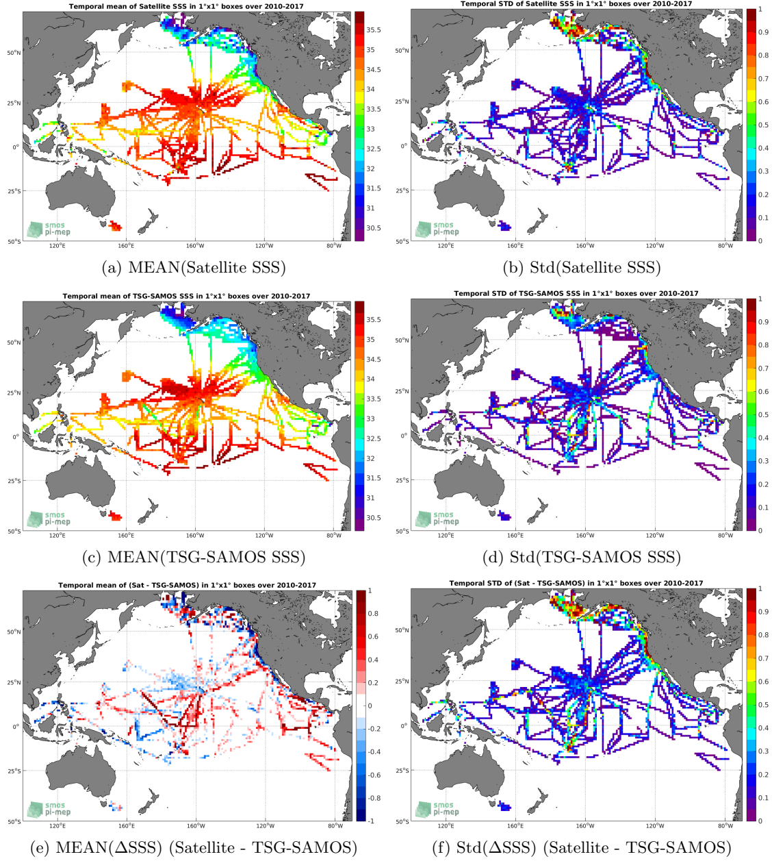
Figure 6: Temporal mean (left) and Std (right) of SSS from SMOS L3 v2 - Monthly - 0.25 Deg (CATDS-CECOS-IFREMER) (top), TSG-SAMOS (middle), and of \Delta SSS (Satellite - TSG-SAMOS). Only match-up pairs are used to generate these maps.
