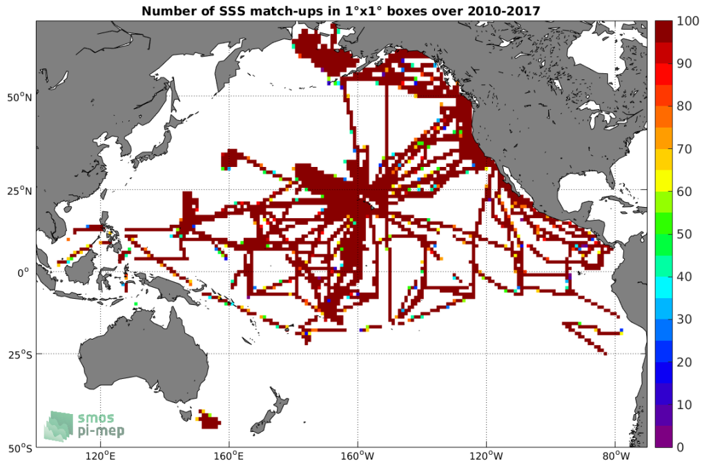
Figure 4: Number of SSS match-ups between TSG-SAMOS SSS and the SMOS L3 v2 - Monthly - 0.25 Deg (CATDS-CECOS-IFREMER) SSS product for the Pacific Ocean Pi-MEP region over 1°x1° boxes and for the full satellite product period.
