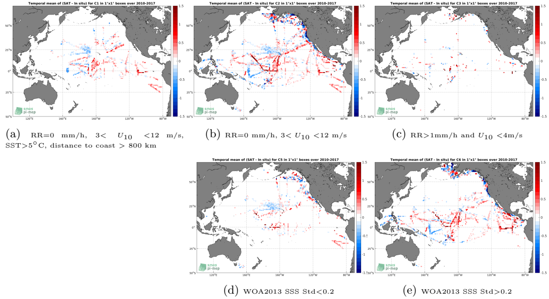
Figure 12: Temporal mean gridded over spatial boxes of size 1^\circ \times 1^\circ of \Delta SSS (SMOS L3 v2 - Monthly - 0.25 Deg (CATDS-CECOS-IFREMER) - TSG-SAMOS) for 5 different subdatasets corresponding to: RR=0 mm/h, 3 < U_{10} < 12 m/s, SST > 5^\circ C , distance to coast > 800 km (a), RR=0 mm/h, 3 < U_{10} < 12 m/s (b), RR > 1 mm/h and U_{10} < 4 m/s (c), WOA2013 SSS Std < 0.2 (d), WOA2013 SSS Std > 0.2 (e).
