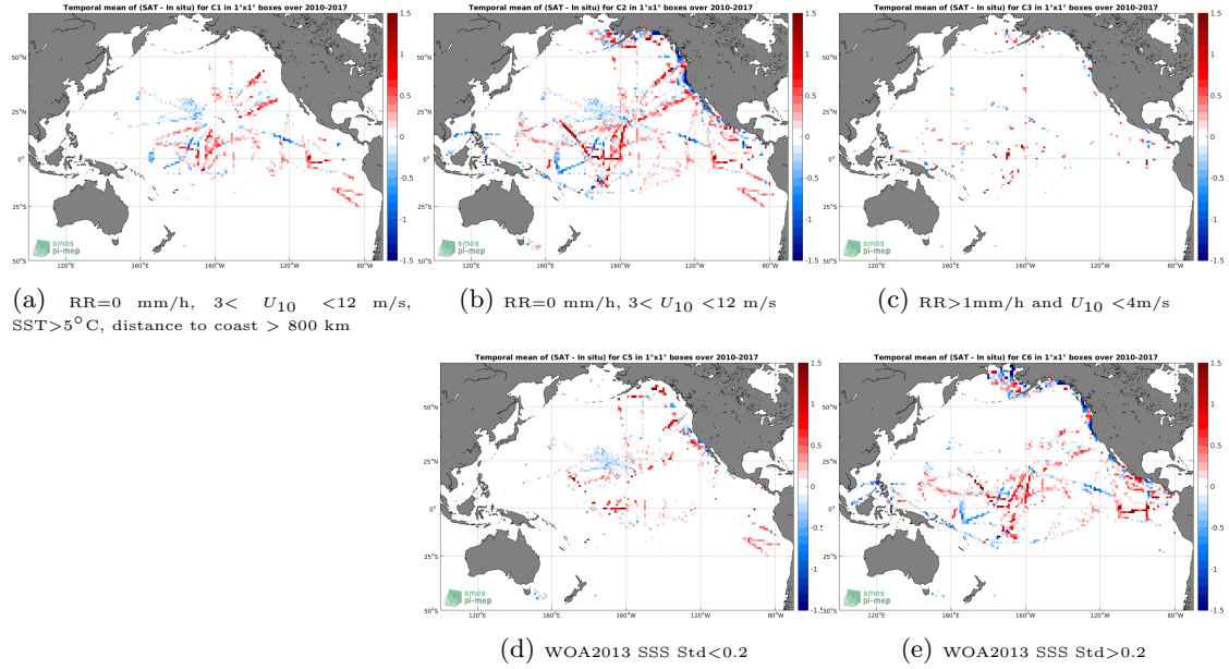
Figure 12: Temporal mean gridded over spatial boxes of size 1^\circ \times 1^\circ of \Delta SSS (SMOS-L3-CATDS-IFREMER-CECOS-V2-MONTHLY-0.25DEG - TSG-SAMOS) for 5 different subdatasets corresponding to:RR=0 mm/h, 3 < U_{10} < 12 m/s, SST >5^\circ\text{C} , distance to coast > 800 km (a), RR=0 mm/h, 3 < U_{10} < 12 m/s (b), RR >1 mm/h and U_{10} < 4 m/s (c), WOA2013 SSS Std <0.2 (d), WOA2013 SSS Std >0.2 (e).
