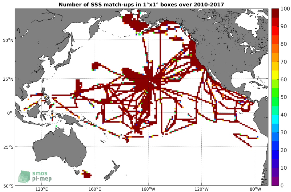
Figure 4: Number of SSS match-ups between TSG-SAMOS SSS and the SMOS-L3-CATDS-IFREMER-CECOS-V2-MONTHLY-0.25DEG SSS product for the Pacific Ocean Pi-MEP region over 1°x1° boxes and for the full satellite product period.
