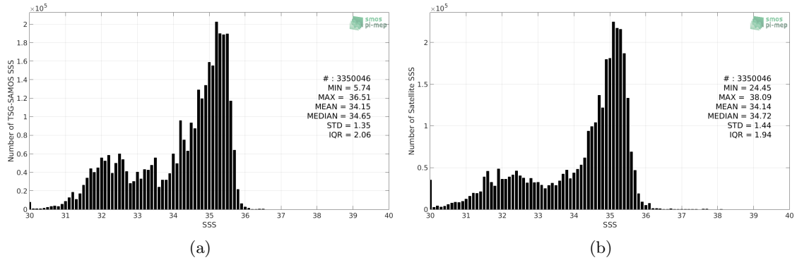
Figure 2: Histograms of SSS from TSG-SAMOS (a) and SMOS-L3-CATDS-IFREMER-CECOS-V2-MONTHLY-0.25DEG (b) considering all match-up pairs per bins of 0.1 over the Pacific Ocean Pi-MEP region and for the full satellite product period.
