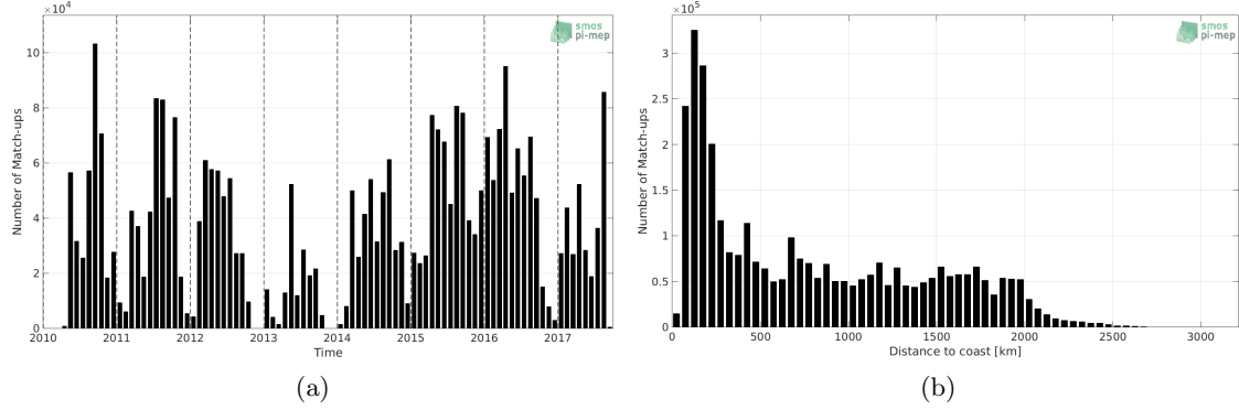
Figure 1: Number of match-ups between TSG-SAMOS and SMOS-L3-CATDS-IFREMER-CECOS-V2-MONTHLY-0.25DEG SSS as a function of time (a) and as function of the distance to coast (b) over the Pacific Ocean Pi-MEP region and for the full satellite product period.
