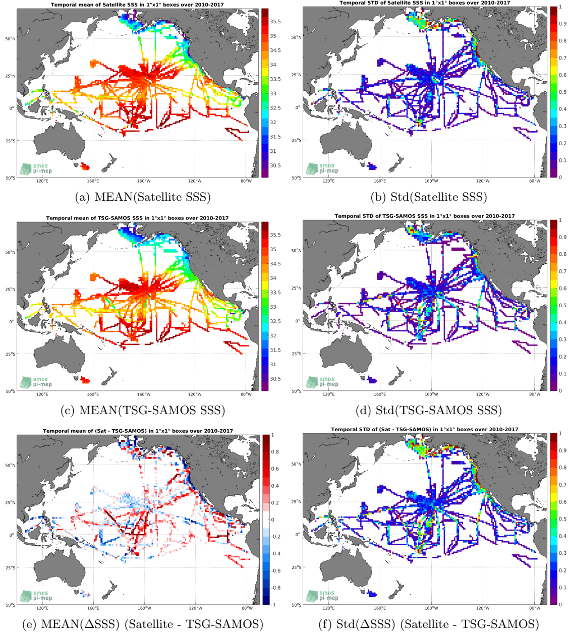
Figure 6: Temporal mean (left) and Std (right) of SSS from SMOS-L3-CATDS-IFREMER-CECOS-V2-MONTHLY-0.25DEG (top), TSG-SAMOS (middle), and of \Delta SSS (Satellite - TSG-SAMOS). Only match-up pairs are used to generate these maps.
