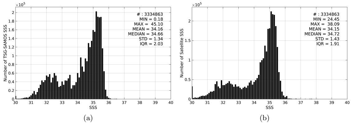
Figure 2: Histograms of SSS from TSG-SAMOS (a) and SMOS-L3-CATDS-IFREMER-CECOS-V2-MONTHLY-0.25DEG (b) considering all match-up pairs per bins of 0.1 over the Pacific Ocean Pi-MEP region and for the full satellite product period.
