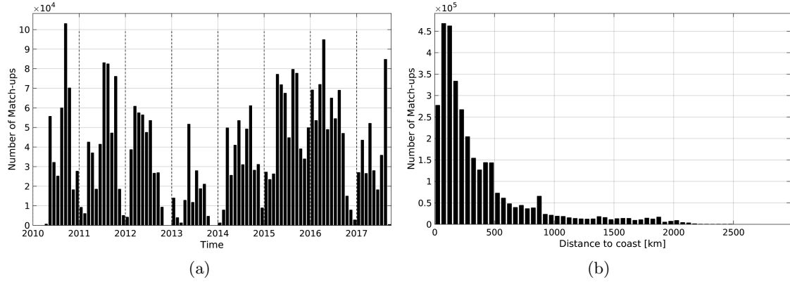
Figure 1: Number of match-ups between TSG-SAMOS and SMOS-L3-CATDS-IFREMER-CECOS-V2-MONTHLY-0.25DEG SSS as a function of time (a) and as function of the distance to coast (b) over the Pacific Ocean Pi-MEP region and for the full satellite product period.
