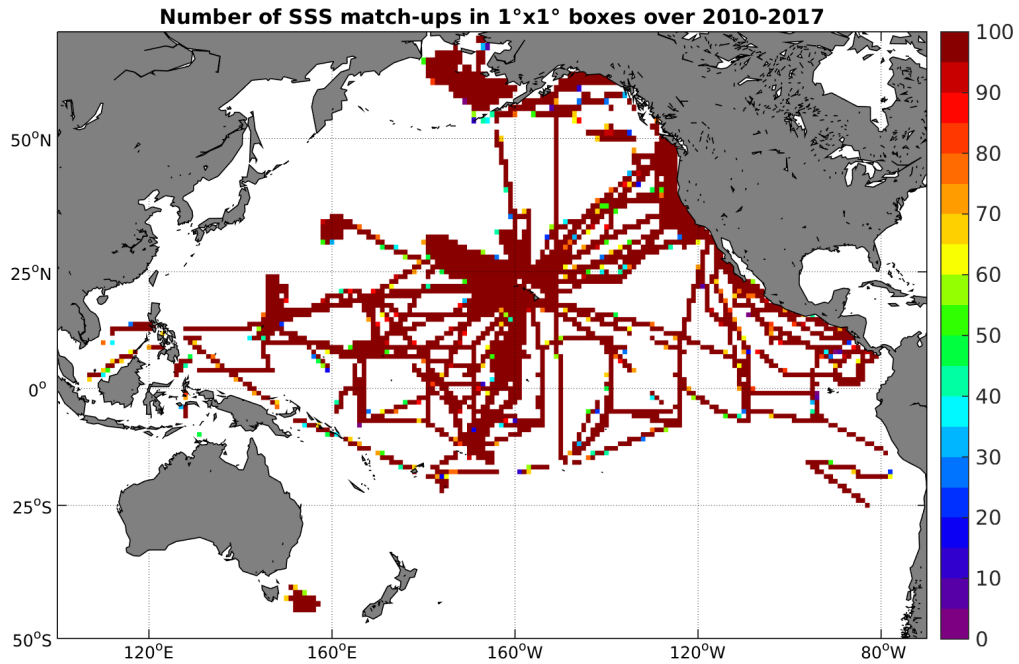
Figure 4: Number of SSS match-ups between TSG-SAMOS SSS and the SMOS-L3-CATDS-IFREMER-CECOS-V2-MONTHLY-0.25DEG SSS product for the Pacific Ocean Pi-MEP region over 1^\circ \times 1^\circ boxes and for the full satellite product period.
