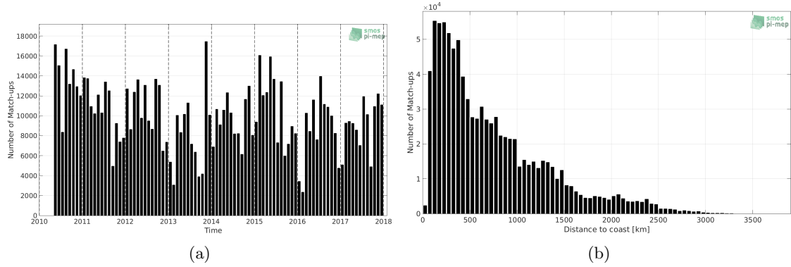
Figure 1: Number of match-ups between TSG (LEGOS-DM) and SMOS SSS L3 v2 - Monthly - 0.25 Deg (CATDS-CECOS-IFREMER) SSS as a function of time (a) and as function of the distance to coast (b) over the Pacific Ocean Pi-MEP region and for the full satellite product period.
