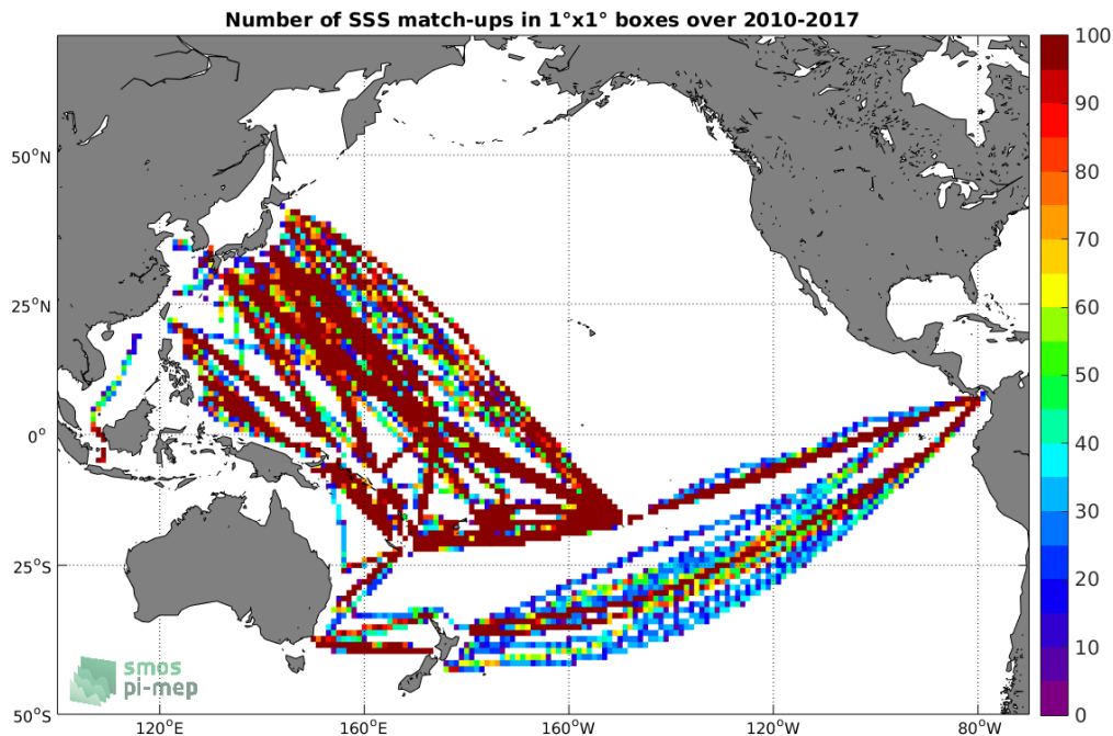
Figure 4: Number of SSS match-ups between TSG (LEGOS-DM) SSS and the SMOS SSS L3 v2 - Monthly - 0.25 Deg (CATDS-CECOS-IFREMER) SSS product for the Pacific Ocean Pi-MEP region over 1^\circ \times 1^\circ boxes and for the full satellite product period.
