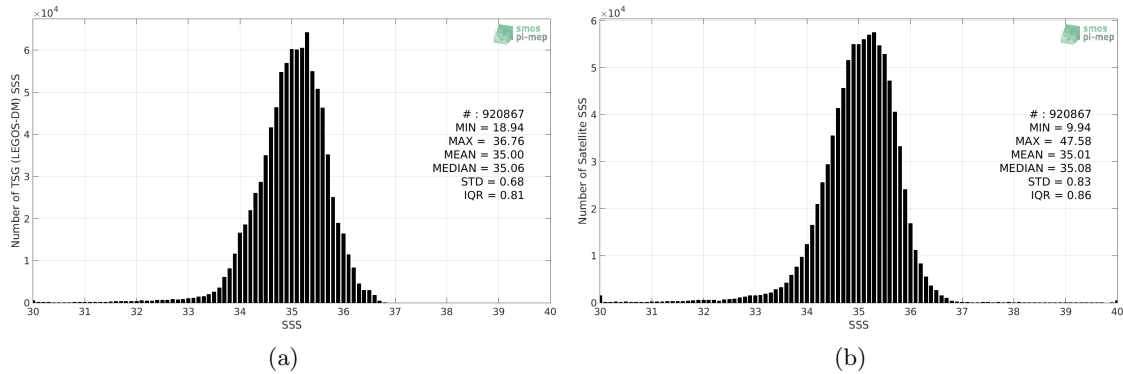
Figure 2: Histograms of SSS from TSG (LEGOS-DM) (a) and SMOS SSS L3 v2 - Monthly - 0.25 Deg (CATDS-CECOS-IFREMER) (b) considering all match-up pairs per bins of 0.1 over the Pacific Ocean Pi-MEP region and for the full satellite product period.
