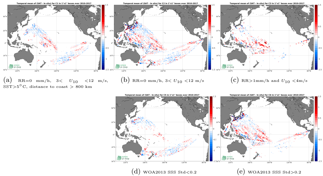
Figure 12: Temporal mean gridded over spatial boxes of size 1^\circ \times 1^\circ of \Delta SSS (SMOS L3 v2 - Monthly - 0.25 Deg (CATDS-CECOS-IFREMER) - TSG-LEGOS-DM) for 5 different subdatasets corresponding to:RR=0 mm/h, 3 < U_{10} < 12 m/s, SST >5^\circ C, distance to coast > 800 km (a), RR=0 mm/h, 3 < U_{10} < 12 m/s (b), RR >1 mm/h and U_{10} < 4 m/s (c), WOA2013 SSS Std <0.2 (d), WOA2013 SSS Std >0.2 (e).
