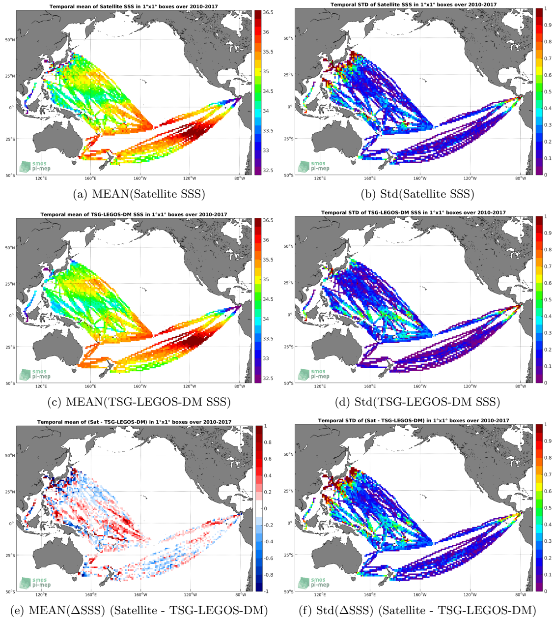
Figure 6: Temporal mean (left) and Std (right) of SSS from SMOS L3 v2 - Monthly - 0.25 Deg (CATDS-CECOS-IFREMER) (top), TSG-LEGOS-DM (middle), and of \Delta SSS (Satellite - TSG-LEGOS-DM). Only match-up pairs are used to generate these maps.
