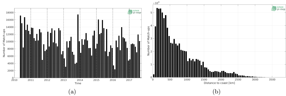
Figure 1: Number of match-ups between TSG-LEGOS-DM and SMOS L3 v2 - Monthly - 0.25 Deg (CATDS-CECOS-IFREMER) SSS as a function of time (a) and as function of the distance to coast (b) over the Pacific Ocean Pi-MEP region and for the full satellite product period.
