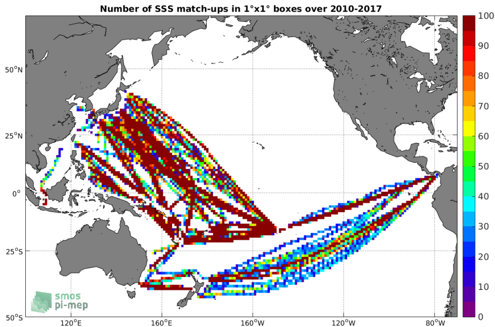
Figure 4: Number of SSS match-ups between TSG-LEGOS-DM SSS and the SMOS L3 v2 - Monthly - 0.25 Deg (CATDS-CECOS-IFREMER) SSS product for the Pacific Ocean Pi-MEP region over 1^\circ \times 1^\circ boxes and for the full satellite product period.
