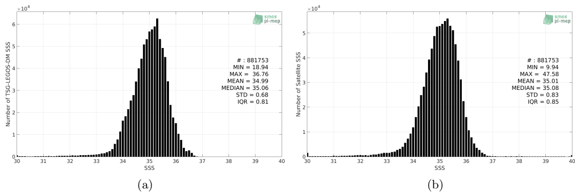
Figure 2: Histograms of SSS from TSG-LEGOS-DM (a) and SMOS L3 v2 - Monthly - 0.25 Deg (CATDS-CECOS-IFREMER) (b) considering all match-up pairs per bins of 0.1 over the Pacific Ocean Pi-MEP region and for the full satellite product period.
