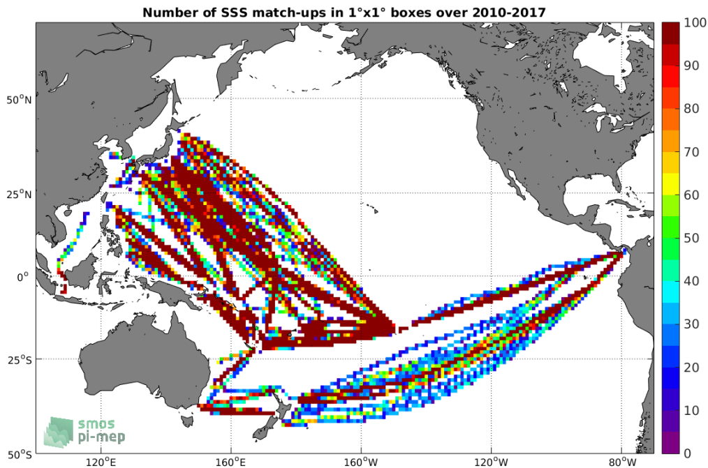
Figure 4: Number of SSS match-ups between TSG-LEGOS-DM SSS and the SMOS-L3-CATDS-IFREMER-CECOS-V2-MONTHLY-0.25DEG SSS product for the Pacific Ocean Pi-MEP region over 1°x1° boxes and for the full satellite product period.
