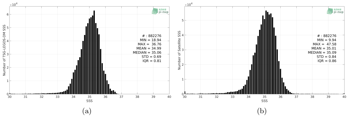
Figure 2: Histograms of SSS from TSG-LEGOS-DM (a) and SMOS-L3-CATDS-IFREMER-CECOS-V2-MONTHLY-0.25DEG (b) considering all match-up pairs per bins of 0.1 over the Pacific Ocean Pi-MEP region and for the full satellite product period.
