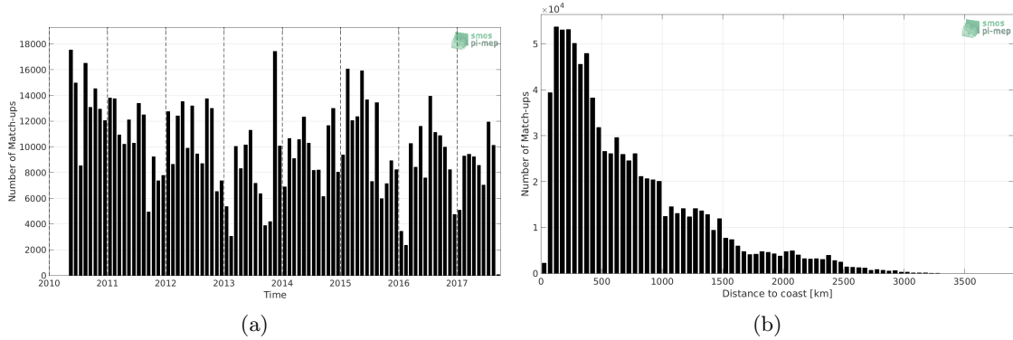
Figure 1: Number of match-ups between TSG-LEGOS-DM and SMOS-L3-CATDS-IFREMER-CECOS-V2-MONTHLY-0.25DEG SSS as a function of time (a) and as function of the distance to coast (b) over the Pacific Ocean Pi-MEP region and for the full satellite product period.
