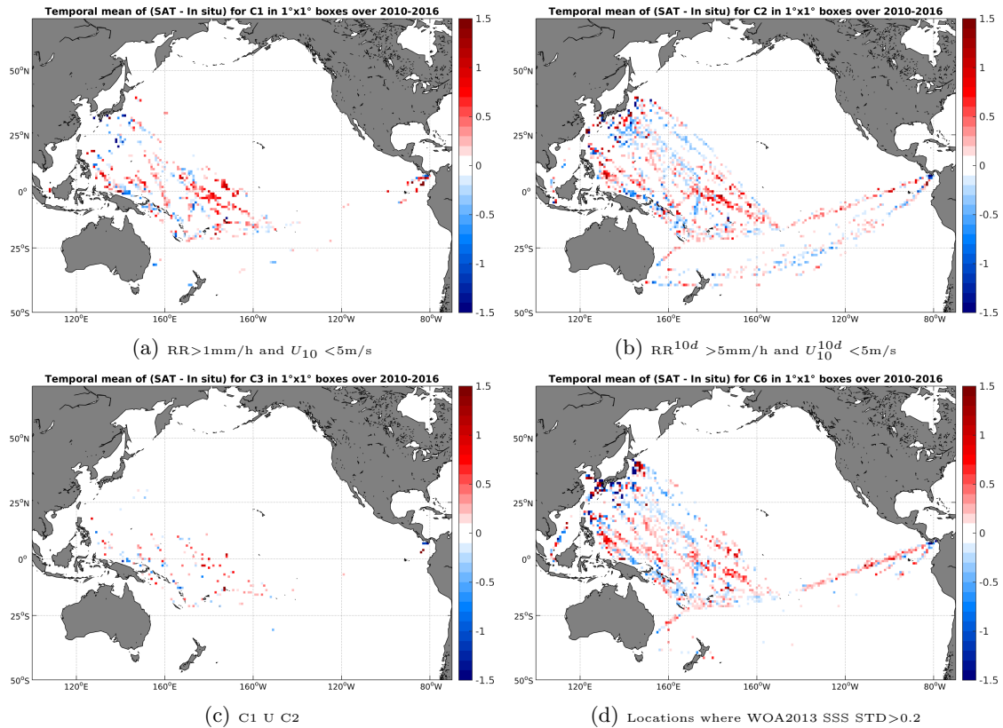
Figure 12: Temporal mean gridded over spatial boxes of size 1^\circ \times 1^\circ of \Delta SSS (SMOS-L3-CATDS-IFREMER-CECOS-V2-MONTHLY-0.25DEG - TSG-LEGOS-DM) for 4 different subdatasets corresponding to:RR>1mm/h and U_{10} < 5\text{m/s} (a), RR^{10d} > 5\text{mm/h} and U_{10}^{10d} < 5\text{m/s} (b), C1 U C2 (c),Locations where WOA2013 SSS STD>0.2 (d).
