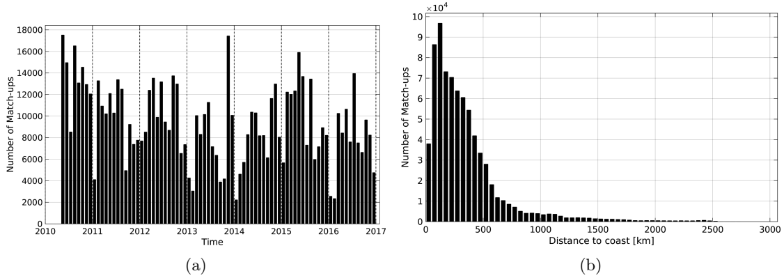
Figure 1: Number of match-ups between TSG-LEGOS-DM and SMOS-L3-CATDS-IFREMER-CECOS-V2-MONTHLY-0.25DEG SSS as a function of time (a) and as function of the distance to coast (b) over the Pacific Ocean Pi-MEP region and for the full satellite product period.
