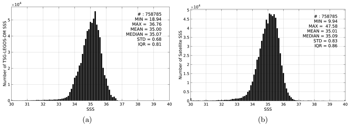
Figure 2: Histograms of SSS from TSG-LEGOS-DM (a) and SMOS-L3-CATDS-IFREMER-CECOS-V2-MONTHLY-0.25DEG (b) considering all match-up pairs per bins of 0.1 over the Pacific Ocean Pi-MEP region and for the full satellite product period.
