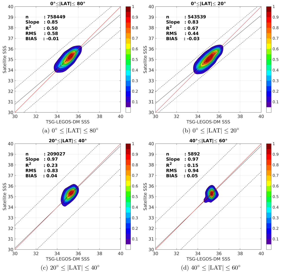
Figure 9: Contour maps of the concentration of SMOS-L3-CATDS-IFREMER-CECOS-V2-MONTHLY-0.25DEG SSS ( y -axis) versus TSG-LEGOS-DM SSS ( x -axis) at match-up pairs for different latitude bands. For each plot, the red line shows x=y . The black thin and dashed lines indicate a linear fit through the data cloud and the \pm 95\% confidence levels, respectively. The number match-up pairs n , the slope and R^2 coefficient of the linear fit, the root mean square (RMS) and the mean bias between satellite and in situ data are indicated for each latitude band in each plots.
