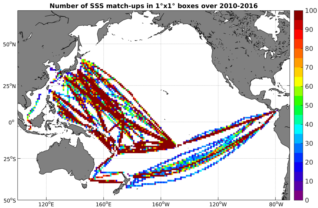
Figure 4: Number of SSS match-ups between TSG-LEGOS-DM SSS and the SMOS-L3-CATDS-IFREMER-CECOS-V2-MONTHLY-0.25DEG SSS product for the Pacific Ocean Pi-MEP region over 1^\circ \times 1^\circ boxes and for the full satellite product period.
