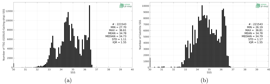
Figure 2: Histograms of SSS from TSG (GOSUD-Sailing-ship) (a) and SMOS SSS L3 v2 - Monthly - 0.25 Deg (CATDS-CECOS-IFREMER) (b) considering all match-up pairs per bins of 0.1 over the Pacific Ocean Pi-MEP region and for the full satellite product period.
