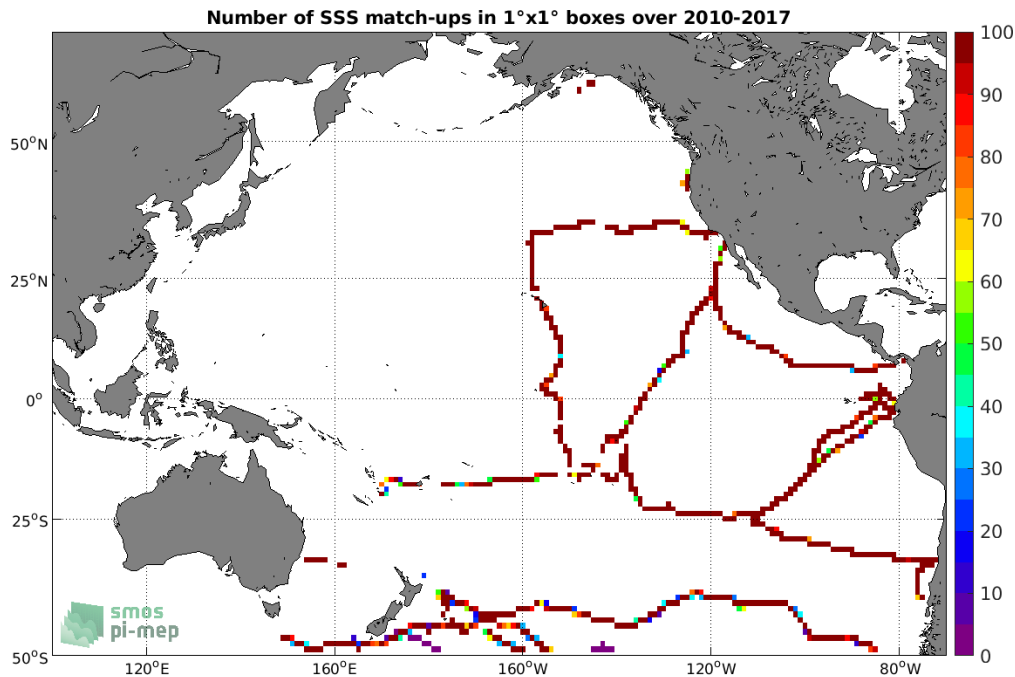
Figure 4: Number of SSS match-ups between TSG (GOSUD-Sailing-ship) SSS and the SMOS SSS L3 v2 - Monthly - 0.25 Deg (CATDS-CECOS-IFREMER) SSS product for the Pacific Ocean Pi-MEP region over 1^\circ \times 1^\circ boxes and for the full satellite product period.
