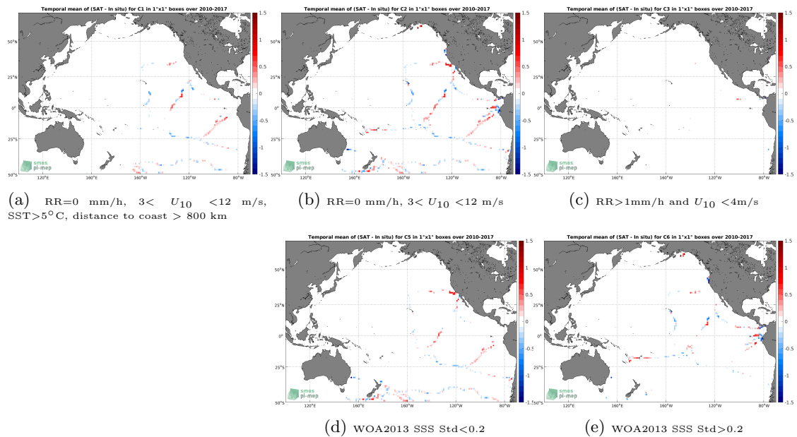
Figure 12: Temporal mean gridded over spatial boxes of size 1^\circ \times 1^\circ of \Delta SSS (SMOS SSS L3 v2 - Monthly - 0.25 Deg (CATDS-CECOS-IFREMER) - TSG (GOSUD-Sailing-ship)) for 5 different subdatasets corresponding to:RR=0 mm/h, 3 < U_{10} < 12 m/s, SST >5^\circ C, distance to coast > 800 km (a), RR=0 mm/h, 3 < U_{10} < 12 m/s (b), RR >1 mm/h and U_{10} < 4 m/s (c), WOA2013 SSS Std <0.2 (d), WOA2013 SSS Std >0.2 (e).
