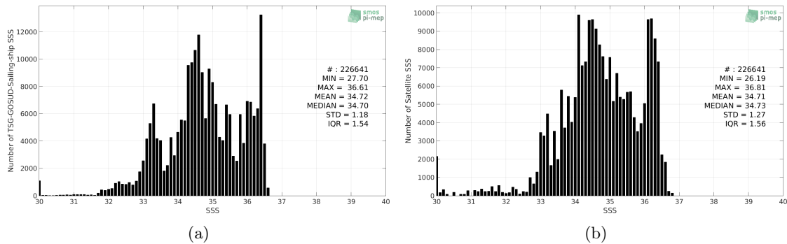
Figure 2: Histograms of SSS from TSG-GOSUD-Sailing-ship (a) and SMOS L3 v2 - Monthly - 0.25 Deg (CATDS-CECOS-IFREMER) (b) considering all match-up pairs per bins of 0.1 over the Pacific Ocean Pi-MEP region and for the full satellite product period.
