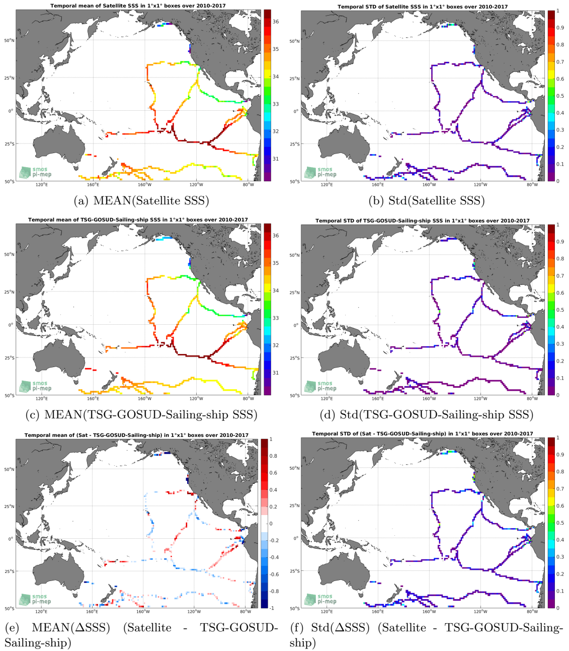
Figure 6: Temporal mean (left) and Std (right) of SSS from SMOS L3 v2 - Monthly - 0.25 Deg (CATDS-CECOS-IFREMER) (top), TSG-GOSUD-Sailing-ship (middle), and of \Delta SSS (Satellite - TSG-GOSUD-Sailing-ship). Only match-up pairs are used to generate these maps.
