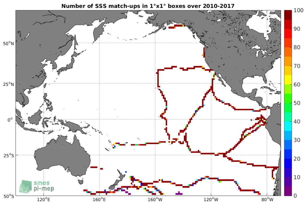
Figure 4: Number of SSS match-ups between TSG-GOSUD-Sailing-ship SSS and the SMOS L3 v2 - Monthly - 0.25 Deg (CATDS-CECOS-IFREMER) SSS product for the Pacific Ocean Pi-MEP region over 1^\circ \times 1^\circ boxes and for the full satellite product period.
