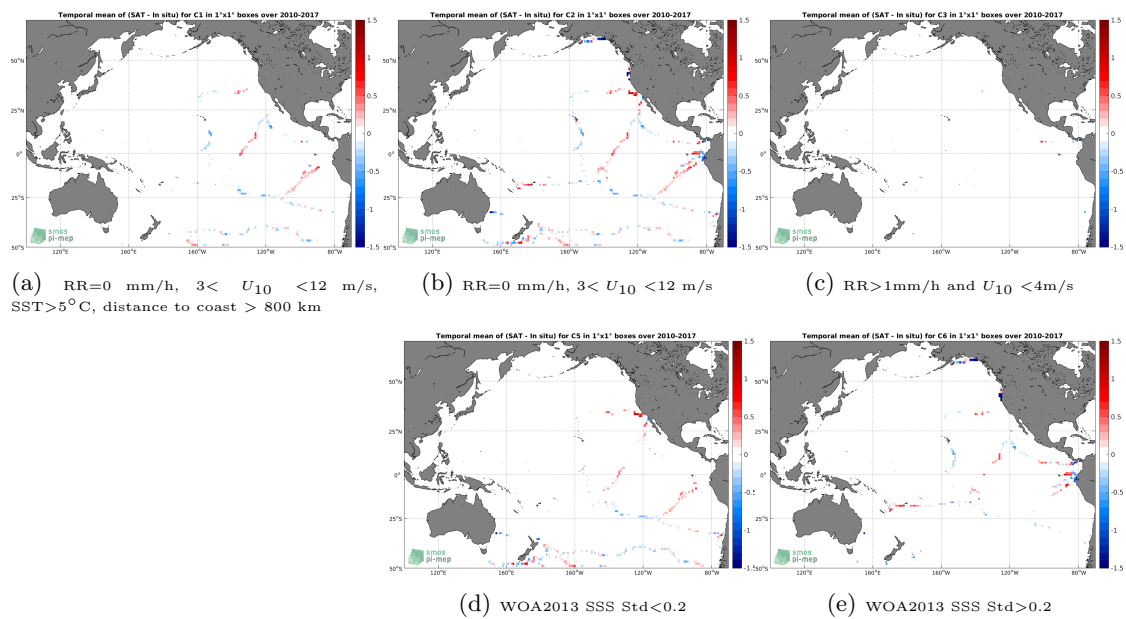
Figure 12: Temporal mean gridded over spatial boxes of size 1^\circ \times 1^\circ of \Delta SSS (SMOS L3 v2 - Monthly - 0.25 Deg (CATDS-CECOS-IFREMER) - TSG-GOSUD-Sailing-ship) for 5 different subdatasets corresponding to:RR=0 mm/h, 3 < U_{10} < 12 m/s, SST > 5^\circ\text{C} , distance to coast > 800 km (a), RR=0 mm/h, 3 < U_{10} < 12 m/s (b), RR > 1 mm/h and U_{10} < 4 m/s (c), WOA2013 SSS Std < 0.2 (d), WOA2013 SSS Std > 0.2 (e).
