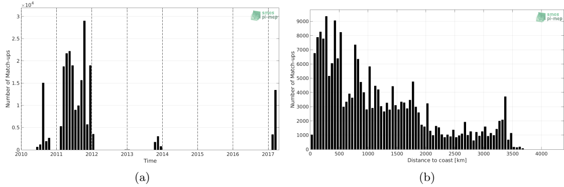
Figure 1: Number of match-ups between TSG-GOSUD-Sailing-ship and SMOS-L3-CATDS-IFREMER-CECOS-V2-MONTHLY-0.25DEG SSS as a function of time (a) and as function of the distance to coast (b) over the Pacific Ocean Pi-MEP region and for the full satellite product period.
