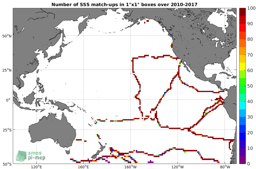
Figure 4: Number of SSS match-ups between TSG-GOSUD-Sailing-ship SSS and the SMOS-L3-CATDS-IFREMER-CECOS-V2-MONTHLY-0.25DEG SSS product for the Pacific Ocean Pi-MEP region over 1^\circ \times 1^\circ boxes and for the full satellite product period.
