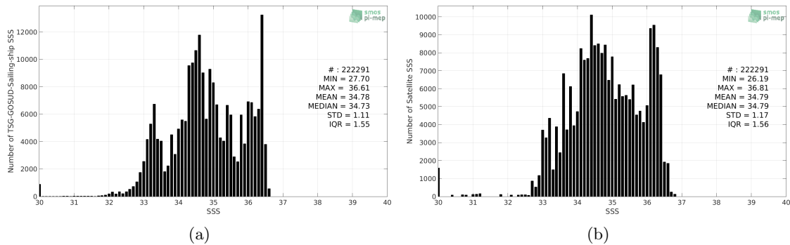
Figure 2: Histograms of SSS from TSG-GOSUD-Sailing-ship (a) and SMOS-L3-CATDS-IFREMER-CECOS-V2-MONTHLY-0.25DEG (b) considering all match-up pairs per bins of 0.1 over the Pacific Ocean Pi-MEP region and for the full satellite product period.
