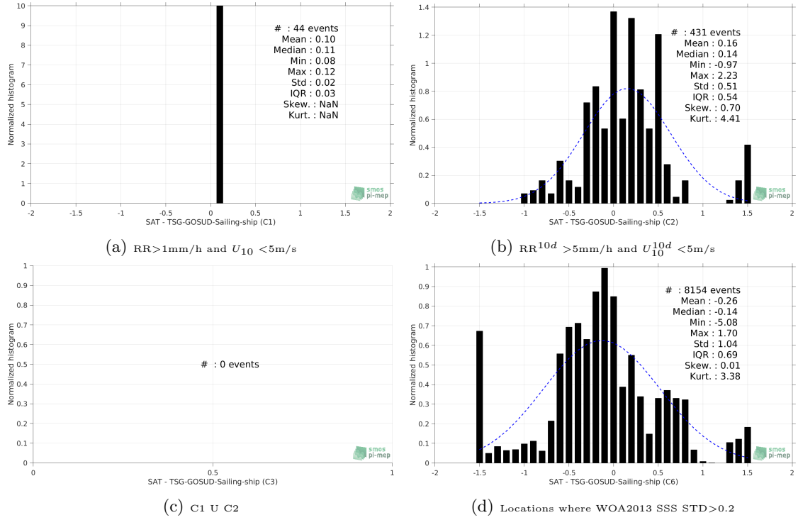
Figure 13: Normalized histogram of \Delta\text{SSS} (SMOS-L3-CATDS-IFREMER-CECOS-V2-MONTHLY-0.25DEG - TSG-GOSUD-Sailing-ship) for 6 different subdatasets corresponding to: RR > 1mm/h and U_{10} < 5\text{m/s} (a), RR^{10d} > 5\text{mm/h} and U_{10}^{10d} < 5\text{m/s} (b), C1 U C2 (c), Locations where WOA2013 SSS STD > 0.2 (d).
