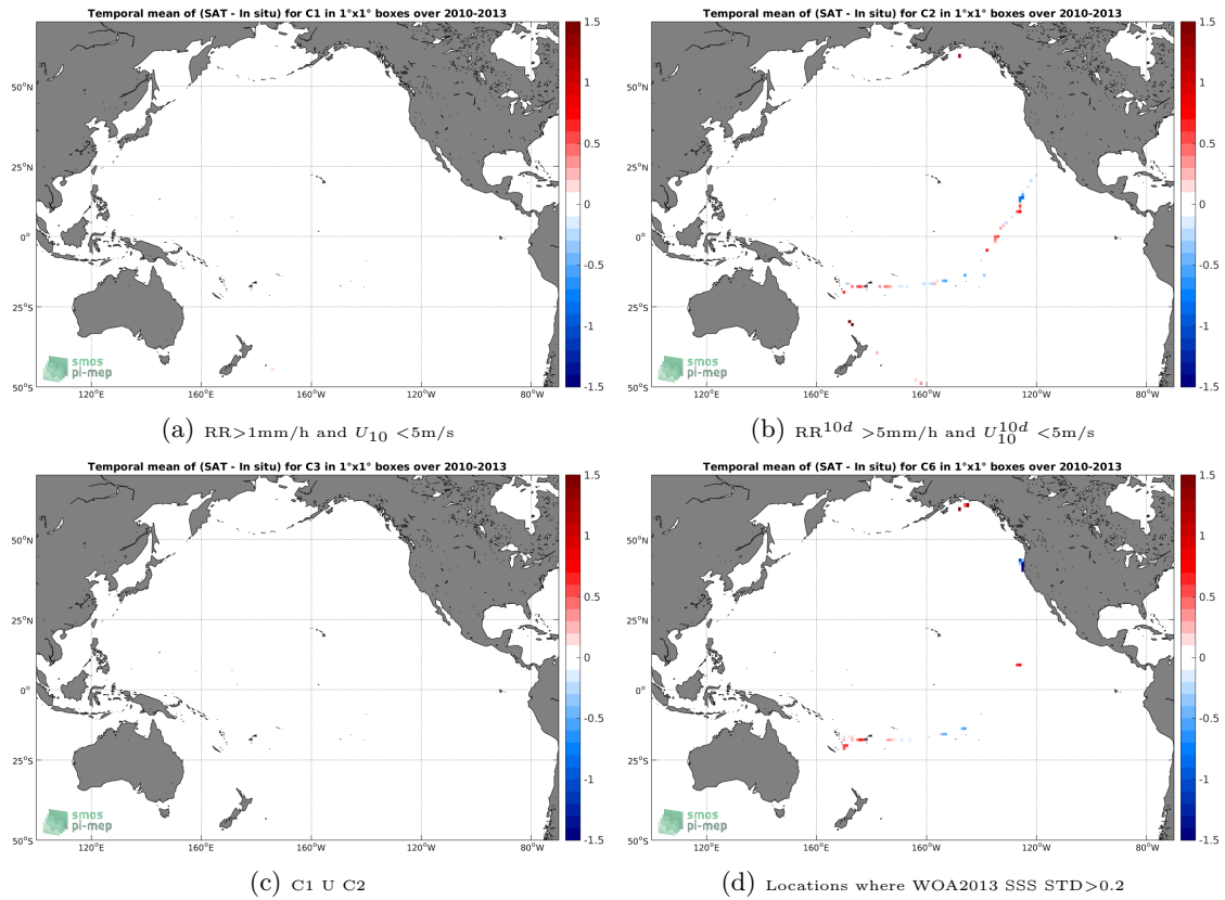
Figure 12: Temporal mean gridded over spatial boxes of size 1^\circ \times 1^\circ of \Delta SSS (SMOS-L3-CATDS-IFREMER-CECOS-V2-MONTHLY-0.25DEG - TSG-GOSUD-Sailing-ship) for 4 different sub-datasets corresponding to: RR > 1\text{mm/h} and U_{10} < 5\text{m/s} (a), RR^{10d} > 5\text{mm/h} and U_{10}^{10d} < 5\text{m/s} (b), C1 U C2 (c), Locations where WOA2013 SSS STD > 0.2 (d).
