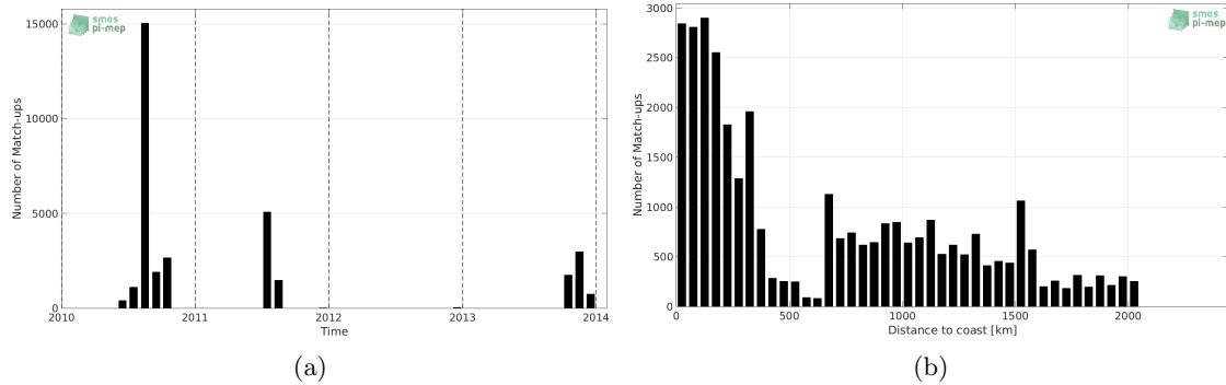
Figure 1: Number of match-ups between TSG-GOSUD-Sailing-ship and SMOS-L3-CATDS-IFREMER-CECOS-V2-MONTHLY-0.25DEG SSS as a function of time (a) and as function of the distance to coast (b) over the Pacific Ocean Pi-MEP region and for the full satellite product period.
