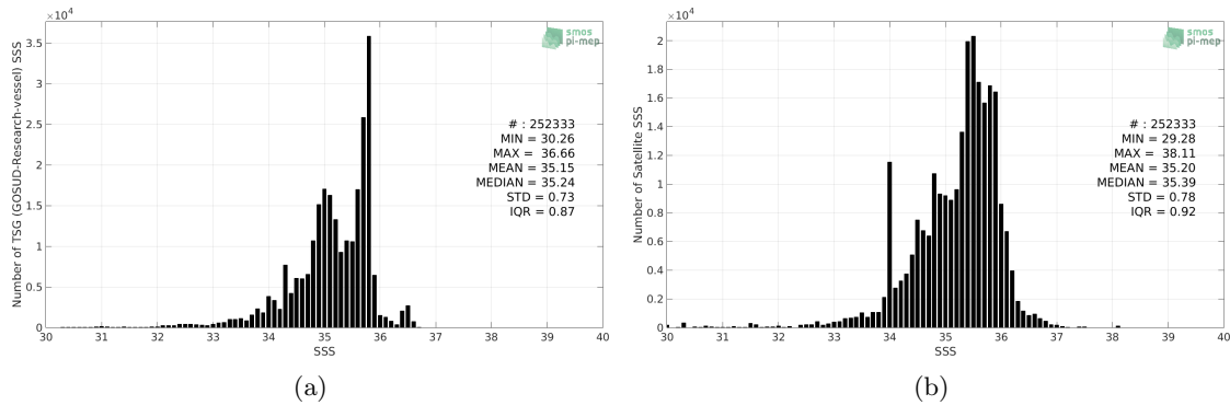
Figure 2: Histograms of SSS from TSG (GOSUD-Research-vessel) (a) and SMOS SSS L3 v2 - Monthly - 0.25 Deg (CATDS-CECOS-IFREMER) (b) considering all match-up pairs per bins of 0.1 over the Pacific Ocean Pi-MEP region and for the full satellite product period.
