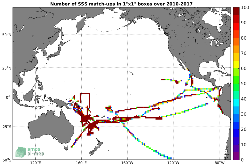
Figure 4: Number of SSS match-ups between TSG (GOSUD-Research-vessel) SSS and the SMOS SSS L3 v2 - Monthly - 0.25 Deg (CATDS-CECOS-IFREMER) SSS product for the Pacific Ocean Pi-MEP region over 1^\circ \times 1^\circ boxes and for the full satellite product period.
