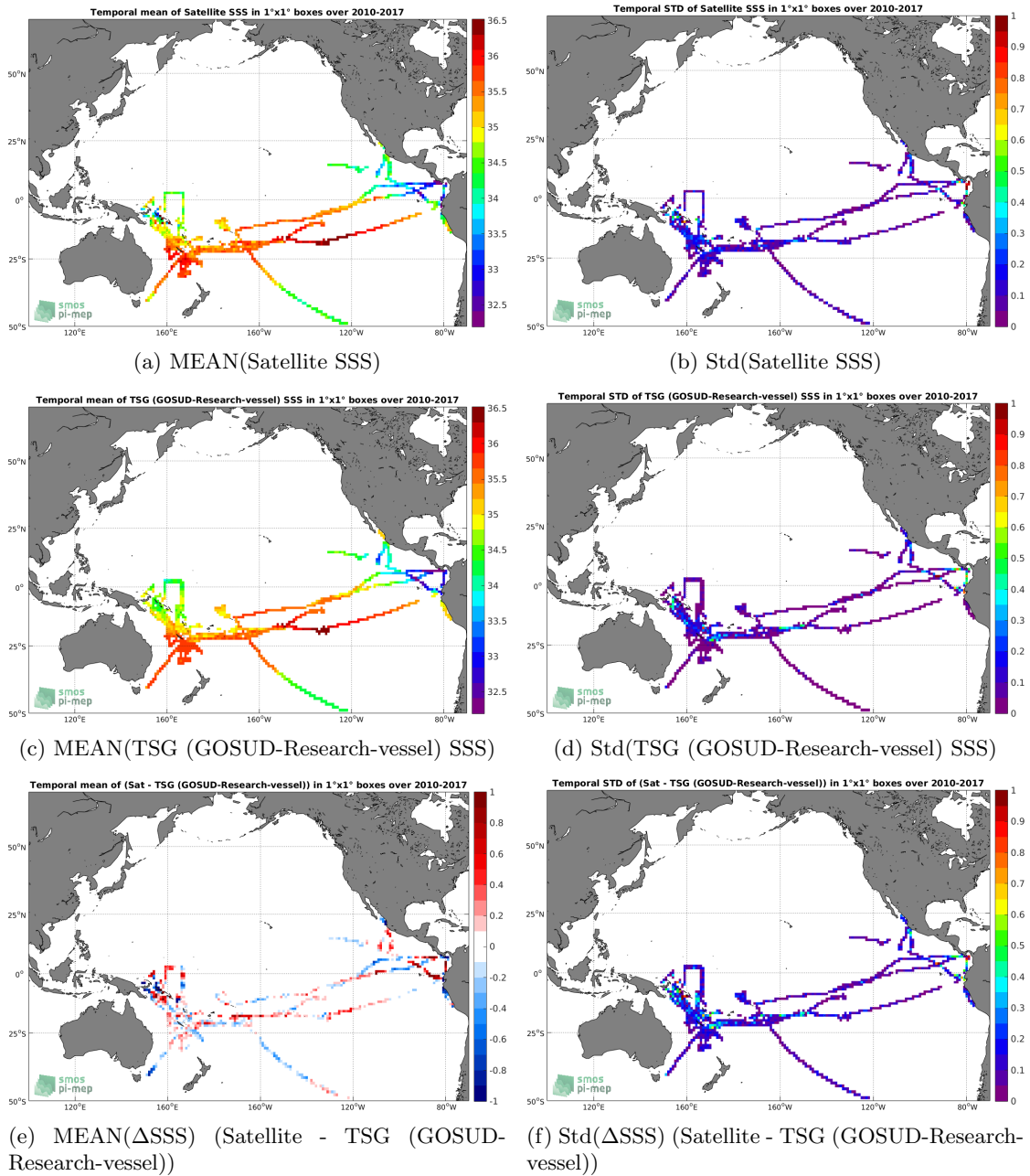
Figure 6: Temporal mean (left) and Std (right) of SSS from SMOS SSS L3 v2 - Monthly - 0.25 Deg (CATDS-CECOS-IFREMER) (top), TSG (GOSUD-Research-vessel) (middle), and of \Delta SSS (Satellite - TSG (GOSUD-Research-vessel)). Only match-up pairs are used to generate these maps.
