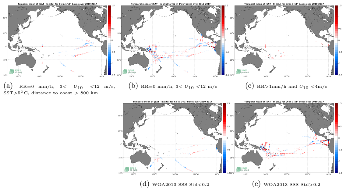
Figure 12: Temporal mean gridded over spatial boxes of size 1^\circ \times 1^\circ of \Delta\text{SSS} (SMOS SSS L3 v2 - Monthly - 0.25 Deg (CATDS-CECOS-IFREMER) - TSG (GOSUD-Research-vessel)) for 5 different subdatasets corresponding to:RR=0 mm/h, 3 < U_{10} < 12 m/s, SST>5°C, distance to coast > 800 km (a), RR=0 mm/h, 3 < U_{10} < 12 m/s (b), RR>1mm/h and U_{10} < 4 m/s (c), WOA2013 SSS Std<0.2 (d), WOA2013 SSS Std>0.2 (e).
