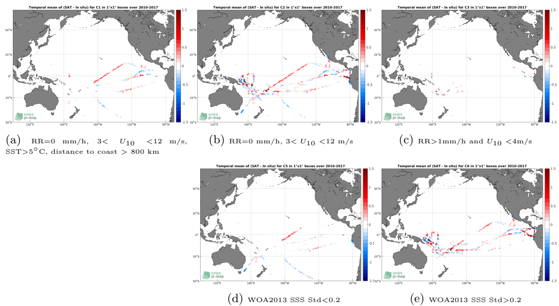
Figure 12: Temporal mean gridded over spatial boxes of size 1^\circ \times 1^\circ of \Delta SSS (SMOS L3 v2 - Monthly - 0.25 Deg (CATDS-CECOS-IFREMER) - TSG-GOSUD-Research-vessel) for 5 different subdatasets corresponding to: RR=0 mm/h, 3 < U_{10} < 12 m/s, SST > 5^\circ C , distance to coast > 800 km (a), RR=0 mm/h, 3 < U_{10} < 12 m/s (b), RR > 1 mm/h and U_{10} < 4 m/s (c), WOA2013 SSS Std < 0.2 (d), WOA2013 SSS Std > 0.2 (e).
