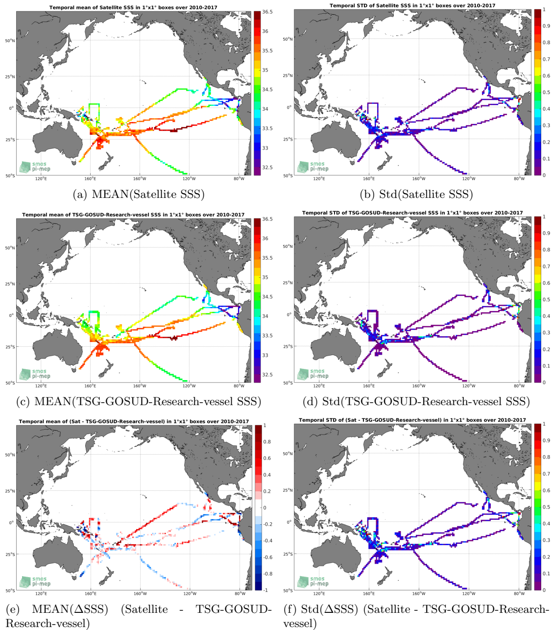
Figure 6: Temporal mean (left) and Std (right) of SSS from SMOS L3 v2 - Monthly - 0.25 Deg (CATDS-CECOS-IFREMER) (top), TSG-GOSUD-Research-vessel (middle), and of \Delta SSS (Satellite - TSG-GOSUD-Research-vessel). Only match-up pairs are used to generate these maps.
