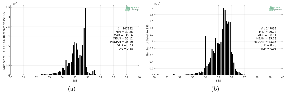
Figure 2: Histograms of SSS from TSG-GOSUD-Research-vessel (a) and SMOS L3 v2 - Monthly - 0.25 Deg (CATDS-CECOS-IFREMER) (b) considering all match-up pairs per bins of 0.1 over the Pacific Ocean Pi-MEP region and for the full satellite product period.
