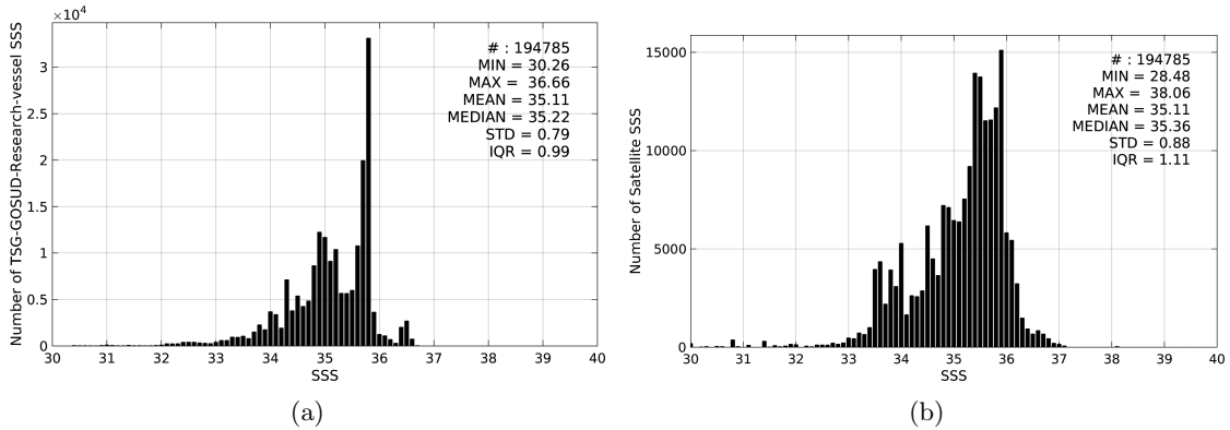
Figure 2: Histograms of SSS from TSG-GOSUD-Research-vessel (a) and SMOS-L3-CATDS-IFREMER-CECOS-V2-MONTHLY-0.25DEG (b) considering all match-up pairs per bins of 0.1 over the Pacific Ocean Pi-MEP region and for the full satellite product period.
