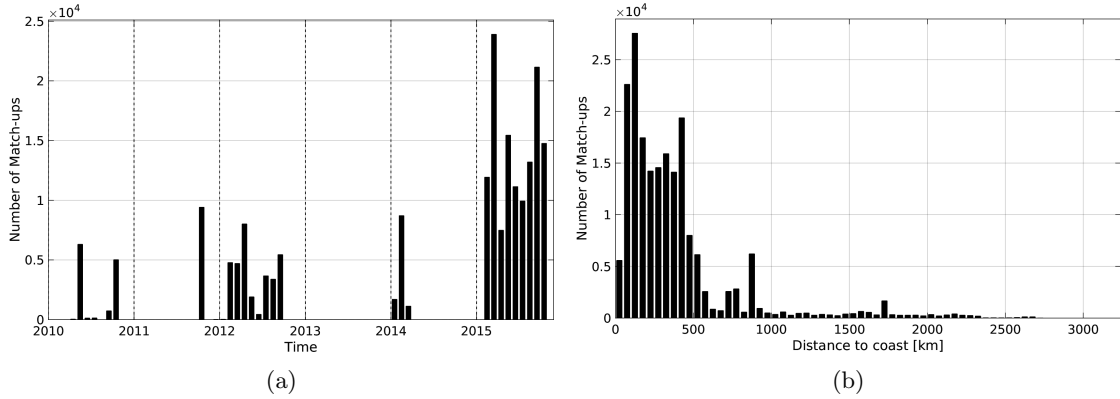
Figure 1: Number of match-ups between TSG-GOSUD-Research-vessel and SMOS-L3-CATDS-IFREMER-CECOS-V2-MONTHLY-0.25DEG SSS as a function of time (a) and as function of the distance to coast (b) over the Pacific Ocean Pi-MEP region and for the full satellite product period.
