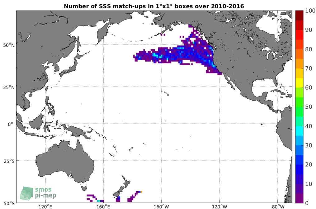
Figure 4: Number of SSS match-ups between Sea mammals SSS and the SMOS SSS L3 v2 - Monthly - 0.25 Deg (CATDS-CECOS-IFREMER) SSS product for the Pacific Ocean Pi-MEP region over 1^\circ \times 1^\circ boxes and for the full satellite product period.
