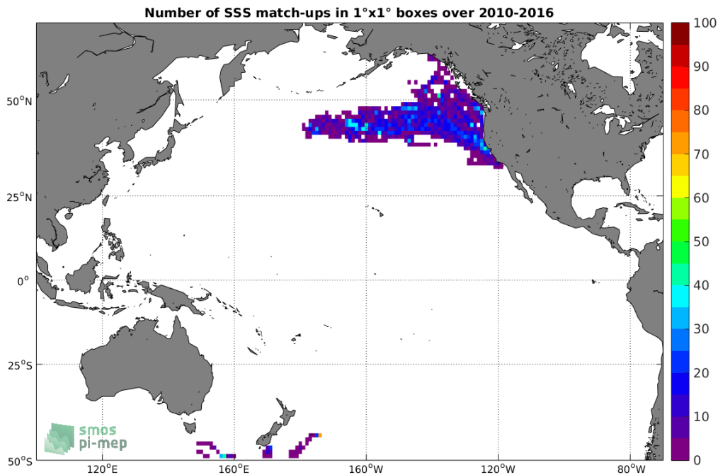
Figure 4: Number of SSS match-ups between Sea mammals SSS and the SMOS-L3-CATDS-IFREMER-CECOS-V2-MONTHLY-0.25DEG SSS product for the Pacific Ocean Pi-MEP region over 1^\circ \times 1^\circ boxes and for the full satellite product period.
