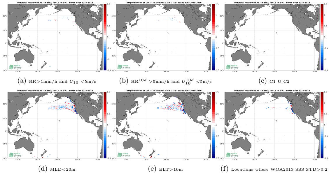
Figure 12: Temporal mean gridded over spatial boxes of size 1^\circ \times 1^\circ of \Delta\text{SSS} (SMOS-L3-CATDS-IFREMER-CECOS-V2-MONTHLY-0.25DEG - Sea mammals) for 6 different subdatasets corresponding to: RR > 1\text{mm/h} and U_{10} < 5\text{m/s} (a), RR^{10d} > 5\text{mm/h} and U_{10}^{10d} < 5\text{m/s} (b), C1 U C2 (c), MLD < 20\text{m} (d), BLT > 10\text{m} (e), Locations where WOA2013 SSS STD > 0.2 (f).
