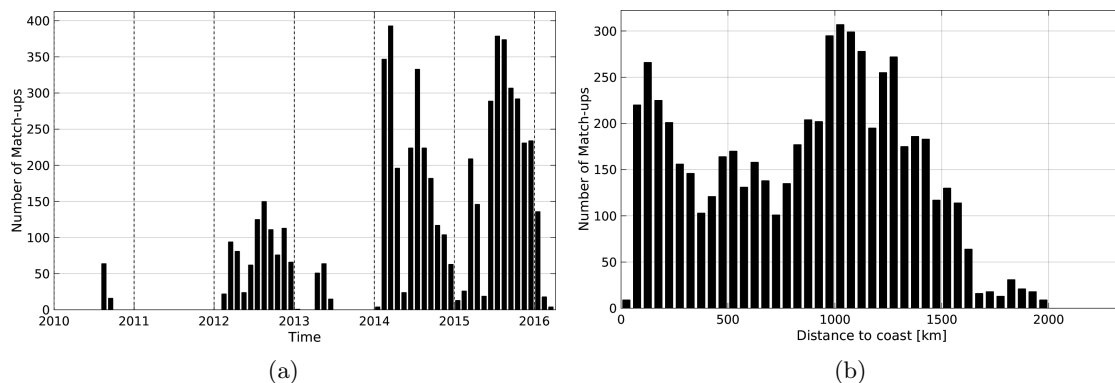
Figure 1: Number of match-ups between Sea mammals and SMOS-L3-CATDS-IFREMER-CECOS-V2-MONTHLY-0.25DEG SSS as a function of time (a) and as function of the distance to coast (b) over the Pacific Ocean Pi-MEP region and for the full satellite product period.
