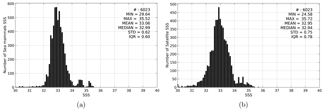
Figure 2: Histograms of SSS from Sea mammals (a) and SMOS-L3-CATDS-IFREMER-CECOS-V2-MONTHLY-0.25DEG (b) considering all match-up pairs per bins of 0.1 over the Pacific Ocean Pi-MEP region and for the full satellite product period.
