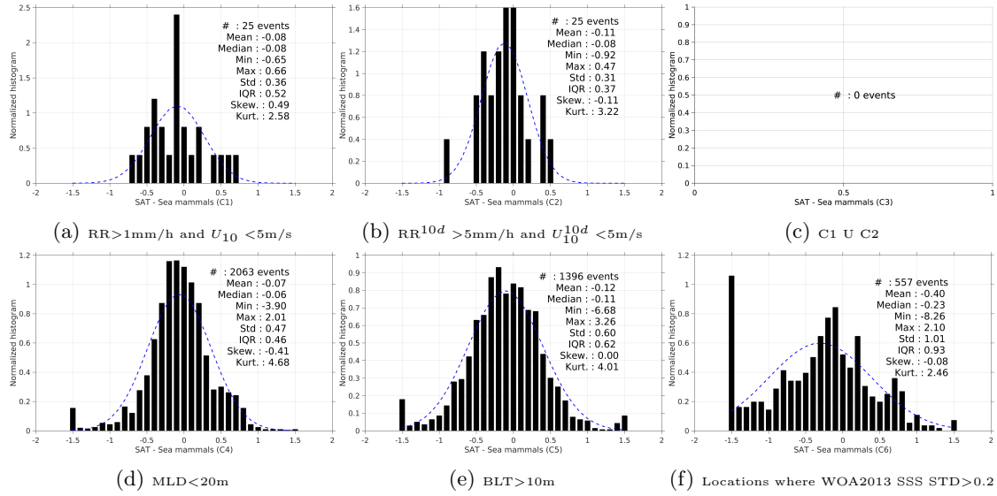
Figure 13: Normalized histogram of \Delta\text{SSS} (SMOS-L3-CATDS-IFREMER-CECOS-V2-MONTHLY-0.25DEG - Sea mammals) for 6 different subdatasets corresponding to: RR > 1mm/h and U_{10} < 5\text{m/s} (a), RR^{10d} > 5\text{mm/h} and U_{10}^{10d} < 5\text{m/s} (b), C1 U C2 (c), MLD < 20m (d), BLT > 10m (e), Locations where WOA2013 SSS STD > 0.2 (f).
