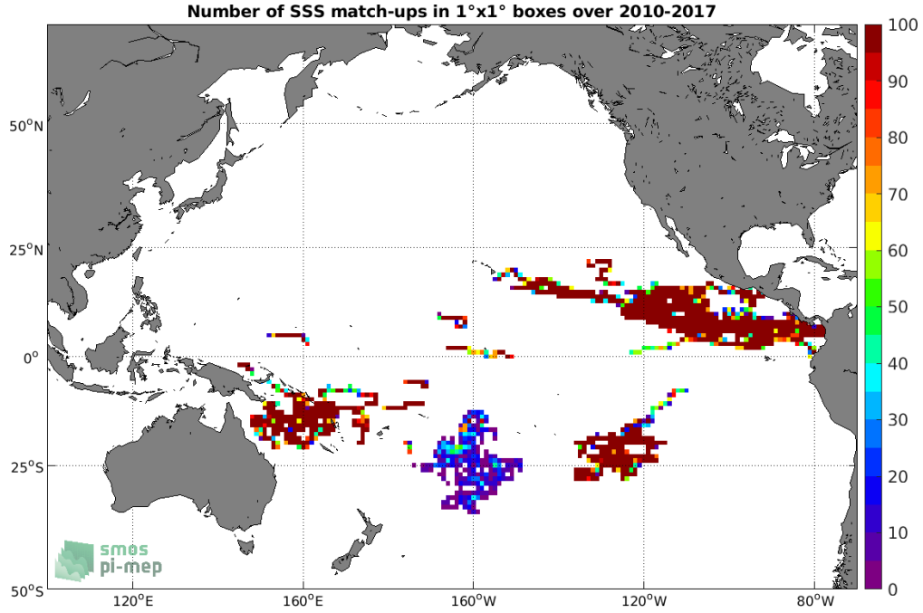
Figure 3: Number of SSS match-ups between Surface drifters SSS and the SMOS SSS L3 v2 - Monthly - 0.25 Deg (CATDS-CECOS-IFREMER) SSS product for the Pacific Ocean Pi-MEP region over 1°x1° boxes and for the full satellite product period.
