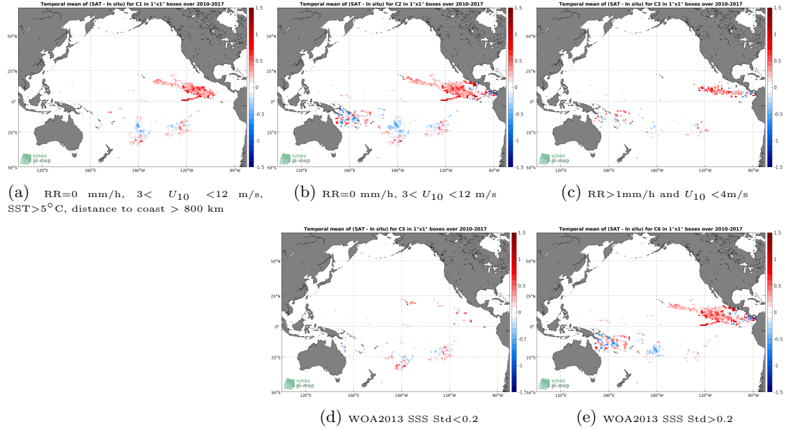
Figure 11: Temporal mean gridded over spatial boxes of size 1^{\circ}\times 1^{\circ} of \Delta\text{SSS} (SMOS SSS L3 v2 - Monthly - 0.25 Deg (CATDS-CECOS-IFREMER) - Surface drifters) for 5 different subdatasets corresponding to:RR=0 mm/h, 3 < U_{10} < 12 m/s, SST >5^{\circ}\text{C} , distance to coast > 800 km (a), RR=0 mm/h, 3 < U_{10} < 12 m/s (b), RR >1 mm/h and U_{10} < 4 m/s (c), WOA2013 SSS Std <0.2 (d), WOA2013 SSS Std >0.2 (e).
