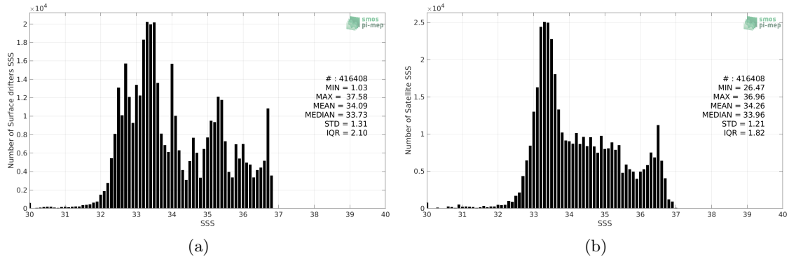
Figure 2: Histograms of SSS from Surface drifters (a) and SMOS SSS L3 v2 - Monthly - 0.25 Deg (CATDS-CECOS-IFREMER) (b) considering all match-up pairs per bins of 0.1 over the Pacific Ocean Pi-MEP region and for the full satellite product period.
