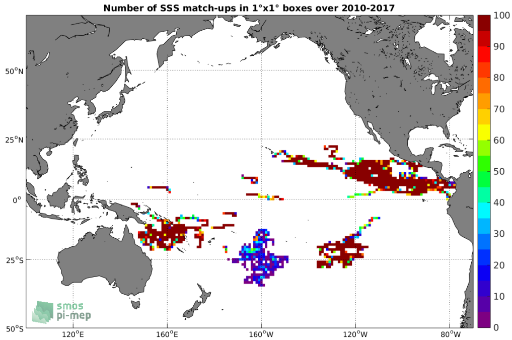
Figure 3: Number of SSS match-ups between Surface drifters SSS and the SMOS L3 v2 - Monthly - 0.25 Deg (CATDS-CECOS-IFREMER) SSS product for the Pacific Ocean Pi-MEP region over 1^\circ \times 1^\circ boxes and for the full satellite product period.
