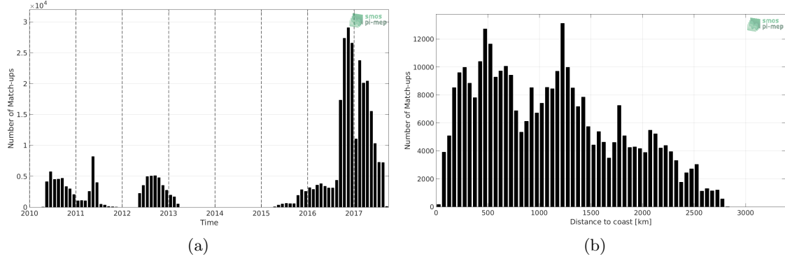
Figure 1: Number of match-ups between Surface drifters and SMOS L3 v2 - Monthly - 0.25 Deg (CATDS-CECOS-IFREMER) SSS as a function of time (a) and as function of the distance to coast (b) over the Pacific Ocean Pi-MEP region and for the full satellite product period.
