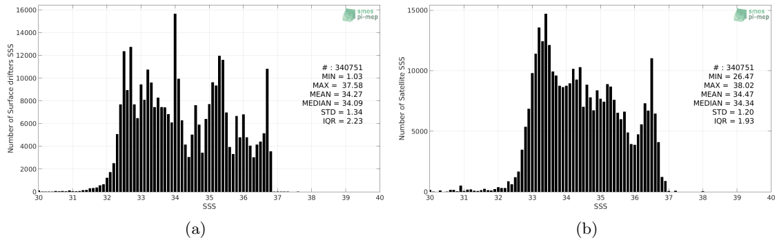
Figure 2: Histograms of SSS from Surface drifters (a) and SMOS L3 v2 - Monthly - 0.25 Deg (CATDS-CECOS-IFREMER) (b) considering all match-up pairs per bins of 0.1 over the Pacific Ocean Pi-MEP region and for the full satellite product period.
