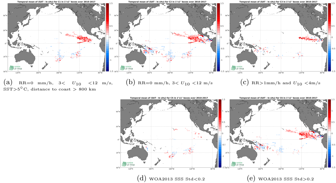
Figure 11: Temporal mean gridded over spatial boxes of size 1^{\circ}\times 1^{\circ} of \Delta\text{SSS} (SMOS L3 v2 - Monthly - 0.25 Deg (CATDS-CECOS-IFREMER) - Surface drifters) for 5 different subdatasets corresponding to: \text{RR}=0 mm/h, 3 < U_{10} < 12 m/s, SST > 5^{\circ}\text{C} , distance to coast > 800 km (a), \text{RR}=0 mm/h, 3 < U_{10} < 12 m/s (b), \text{RR}>1\text{mm/h} and U_{10} < 4\text{m/s} (c), WOA2013 SSS Std < 0.2 (d), WOA2013 SSS Std > 0.2 (e).
