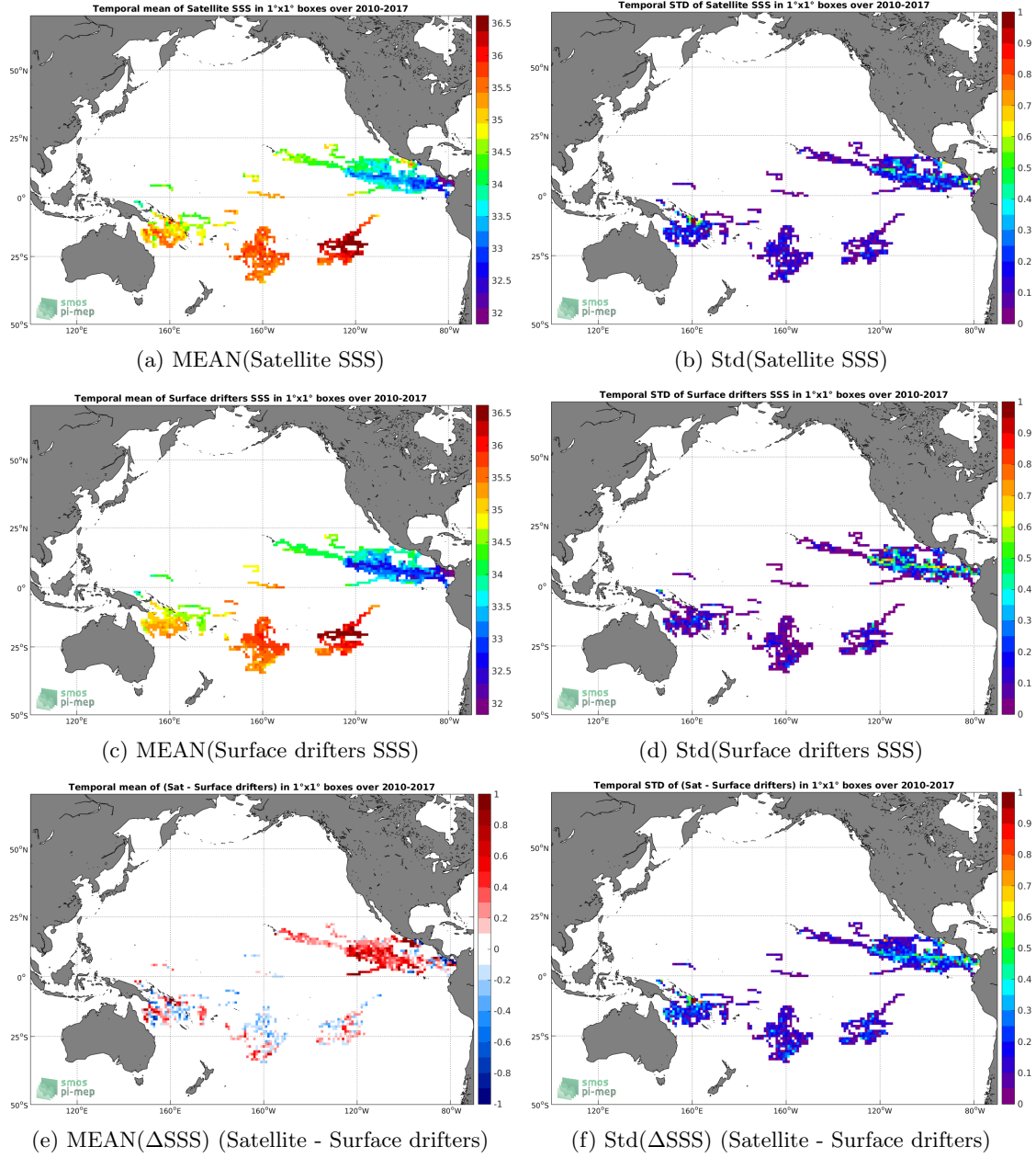
Figure 5: Temporal mean (left) and Std (right) of SSS from SMOS L3 v2 - Monthly - 0.25 Deg (CATDS-CECOS-IFREMER) (top), Surface drifters (middle), and of \Delta SSS (Satellite - Surface drifters). Only match-up pairs are used to generate these maps.
