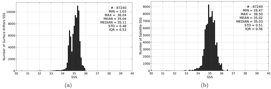
Figure 2: Histograms of SSS from Surface drifters (a) and SMOS-L3-CATDS-IFREMER-CECOS-V2-MONTHLY-0.25DEG (b) considering all match-up pairs per bins of 0.1 over the Pacific Ocean Pi-MEP region and for the full satellite product period.
