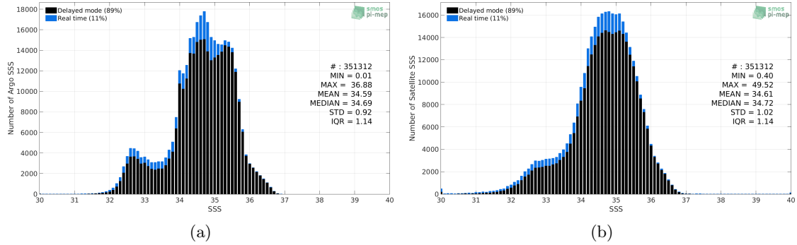
Figure 2: Histograms of SSS from Argo (a) and SMOS SSS L3 v2 - Monthly - 0.25 Deg (CATDS-CECOS-IFREMER) (b) considering all match-up pairs per bins of 0.1 over the Pacific Ocean Pi-MEP region and for the full satellite product period.
