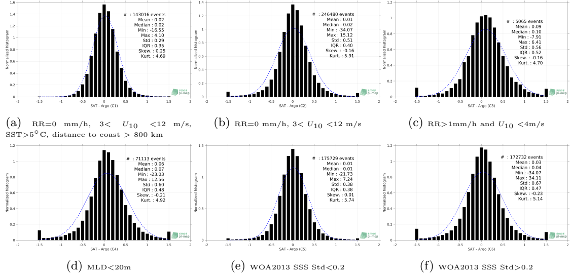
Figure 13: Normalized histogram of \Delta\text{SSS} (SMOS SSS L3 v2 - Monthly - 0.25 Deg (CATDS-CECOS-IFREMER) - Argo) for 6 different subdatasets corresponding to: RR=0 mm/h, 3 < U_{10} < 12 m/s, SST>5°C, distance to coast > 800 km (a), RR=0 mm/h, 3 < U_{10} < 12 m/s (b), RR>1mm/h and U_{10} < 4 m/s (c), MLD<20m (d), WOA2013 SSS Std<0.2 (e), WOA2013 SSS Std>0.2 (f).
