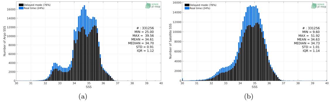
Figure 2: Histograms of SSS from Argo (a) and SMOS-L3-CATDS-IFREMER-CECOS-V2-MONTHLY-0.25DEG (b) considering all match-up pairs per bins of 0.1 over the Pacific Ocean Pi-MEP region and for the full satellite product period.
