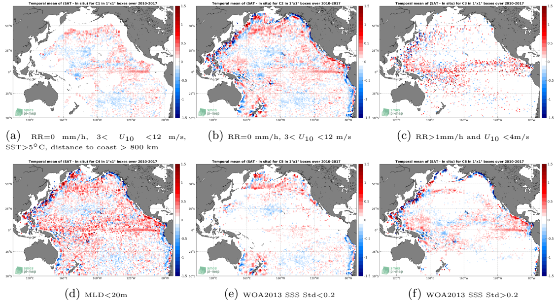
Figure 12: Temporal mean gridded over spatial boxes of size 1^\circ \times 1^\circ of \Delta SSS (SMOS-L3-CATDS-IFREMER-CECOS-V2-MONTHLY-0.25DEG - Argo) for 6 different subdatasets corresponding to: RR=0 mm/h, 3 < U_{10} < 12 m/s, SST > 5^\circ C , distance to coast > 800 km (a), RR=0 mm/h, 3 < U_{10} < 12 m/s (b), RR > 1 mm/h and U_{10} < 4 m/s (c), MLD < 20 m (d), WOA2013 SSS Std < 0.2 (e), WOA2013 SSS Std > 0.2 (f).
