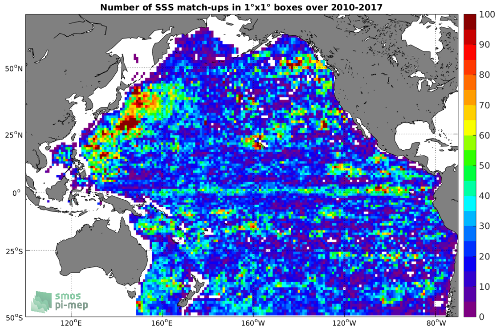
Figure 4: Number of SSS match-ups between Argo SSS and the SMOS-L3-CATDS-IFREMER-CECOS-V2-MONTHLY-0.25DEG SSS product for the Pacific Ocean Pi-MEP region over 1^\circ \times 1^\circ boxes and for the full satellite product period.
