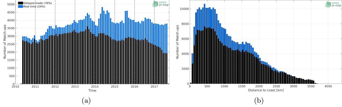
Figure 1: Number of match-ups between Argo and SMOS-L3-CATDS-IFREMER-CECOS-V2-MONTHLY-0.25DEG SSS as a function of time (a) and as function of the distance to coast (b) over the Pacific Ocean Pi-MEP region and for the full satellite product period.
