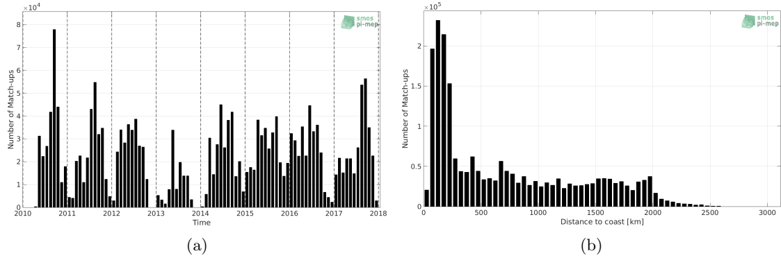
Figure 1: Number of match-ups between TSG (SAMOS) and SMOS SSS L3 v2 - Daily - 0.5 Deg (CATDS-CECOS-IFREMER) SSS as a function of time (a) and as function of the distance to coast (b) over the Pacific Ocean Pi-MEP region and for the full satellite product period.
