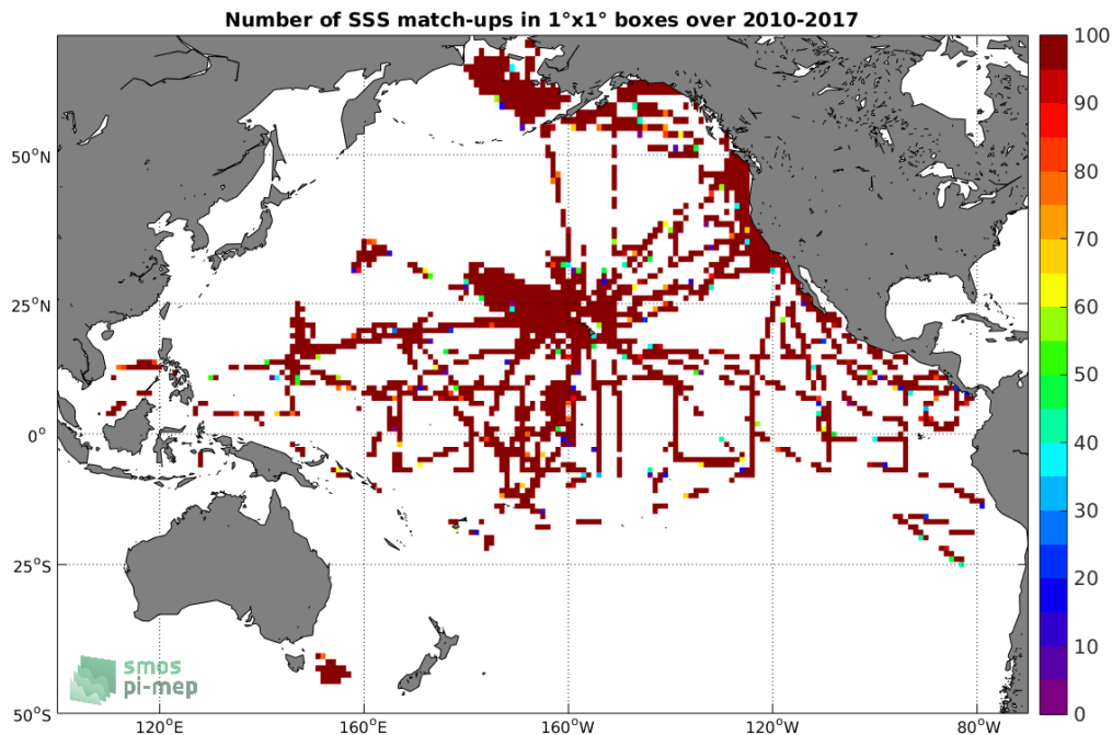
Figure 4: Number of SSS match-ups between TSG (SAMOS) SSS and the SMOS SSS L3 v2 - Daily - 0.5 Deg (CATDS-CECOS-IFREMER) SSS product for the Pacific Ocean Pi-MEP region over 1^\circ \times 1^\circ boxes and for the full satellite product period.
