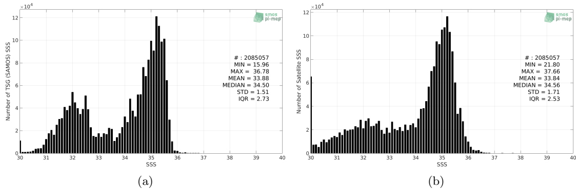
Figure 2: Histograms of SSS from TSG (SAMOS) (a) and SMOS SSS L3 v2 - Daily - 0.5 Deg (CATDS-CECOS-IFREMER) (b) considering all match-up pairs per bins of 0.1 over the Pacific Ocean Pi-MEP region and for the full satellite product period.
