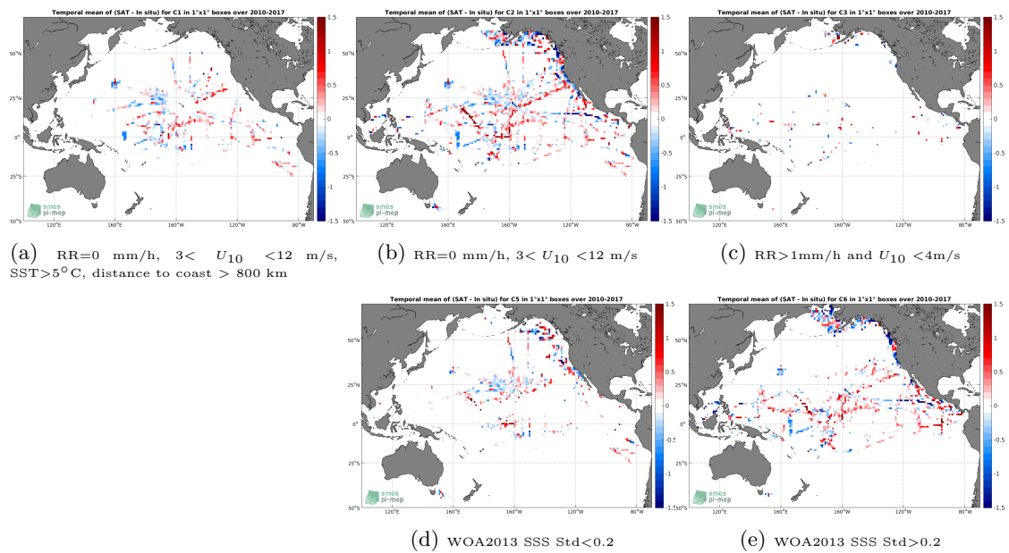
Figure 12: Temporal mean gridded over spatial boxes of size 1^\circ \times 1^\circ of \Delta\text{SSS} (SMOS SSS L3 v2 - Daily - 0.5 Deg (CATDS-CECOS-IFREMER) - TSG (SAMOS)) for 5 different subdatasets corresponding to:RR=0 mm/h, 3 < U_{10} < 12 m/s, SST >5^\circ\text{C} , distance to coast > 800 km (a), RR=0 mm/h, 3 < U_{10} < 12 m/s (b), RR >1 mm/h and U_{10} < 4 m/s (c), WOA2013 SSS Std <0.2 (d), WOA2013 SSS Std >0.2 (e).
