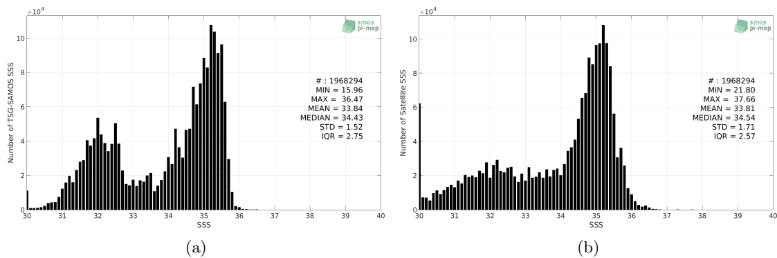
Figure 2: Histograms of SSS from TSG-SAMOS (a) and SMOS L3 v2 - Daily - 0.5 Deg (CATDS-CECOS-IFREMER) (b) considering all match-up pairs per bins of 0.1 over the Pacific Ocean Pi-MEP region and for the full satellite product period.
