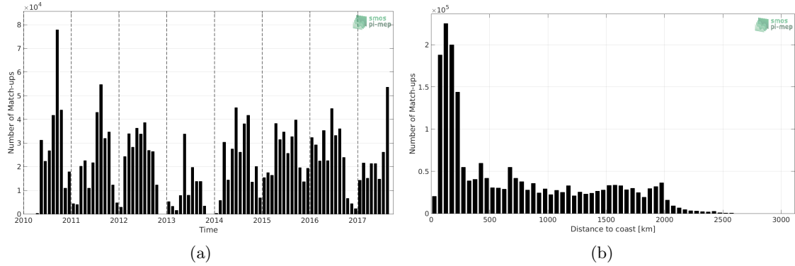
Figure 1: Number of match-ups between TSG-SAMOS and SMOS L3 v2 - Daily - 0.5 Deg (CATDS-CECOS-IFREMER) SSS as a function of time (a) and as function of the distance to coast (b) over the Pacific Ocean Pi-MEP region and for the full satellite product period.
