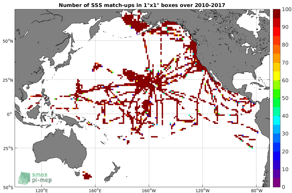
Figure 4: Number of SSS match-ups between TSG-SAMOS SSS and the SMOS L3 v2 - Daily - 0.5 Deg (CATDS-CECOS-IFREMER) SSS product for the Pacific Ocean Pi-MEP region over 1°x1° boxes and for the full satellite product period.
