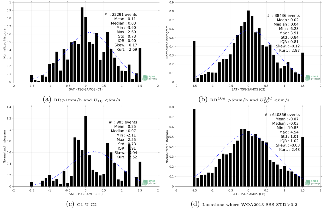
Figure 13: Normalized histogram of \Delta SSS (SMOS-L3-CATDS-CECOS-IFREMER-V2-1DAY-0.5DEG - TSG-SAMOS) for 6 different subdatasets corresponding to: RR > 1\text{mm/h} and U_{10} < 5\text{m/s} (a), RR^{10d} > 5\text{mm/h} and U_{10}^{10d} < 5\text{m/s} (b), C1 U C2 (c), Locations where WOA2013 SSS STD > 0.2 (d).
