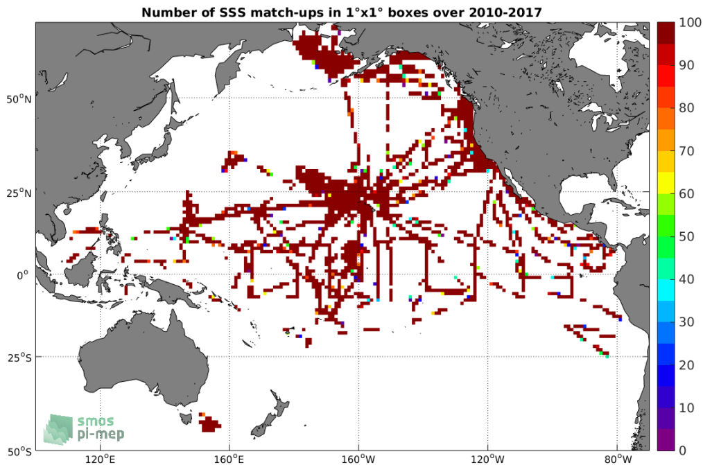
Figure 4: Number of SSS match-ups between TSG-SAMOS SSS and the SMOS-L3-CATDS-CECOS-IFREMER-V2-1DAY-0.5DEG SSS product for the Pacific Ocean Pi-MEP region over 1^\circ \times 1^\circ boxes and for the full satellite product period.
