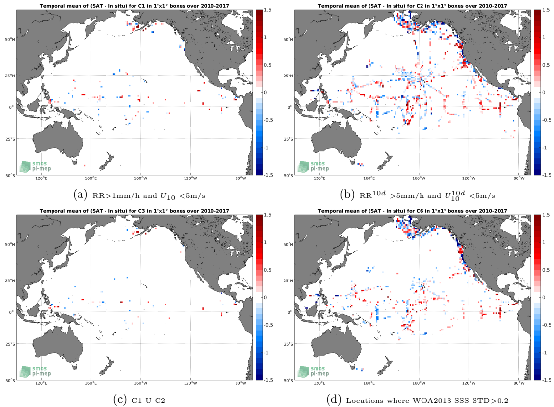
Figure 12: Temporal mean gridded over spatial boxes of size 1^\circ \times 1^\circ of \Delta SSS (SMOS-L3-CATDS-CECOS-IFREMER-V2-1DAY-0.5DEG - TSG-SAMOS) for 4 different subdatasets corresponding to: RR > 1\text{mm/h} and U_{10} < 5\text{m/s} (a), RR^{10d} > 5\text{mm/h} and U_{10}^{10d} < 5\text{m/s} (b), C1 U C2 (c), Locations where WOA2013 SSS STD > 0.2 (d).
