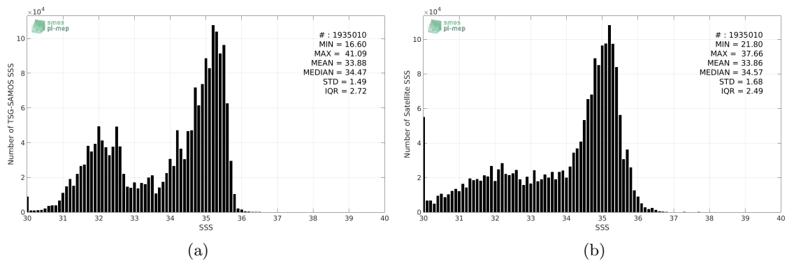
Figure 2: Histograms of SSS from TSG-SAMOS (a) and SMOS-L3-CATDS-CECOS-IFREMER-V2-1DAY-0.5DEG (b) considering all match-up pairs per bins of 0.1 over the Pacific Ocean Pi-MEP region and for the full satellite product period.
