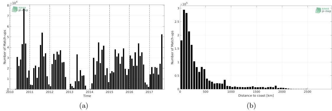
Figure 1: Number of match-ups between TSG-SAMOS and SMOS-L3-CATDS-CECOS-IFREMER-V2-1DAY-0.5DEG SSS as a function of time (a) and as function of the distance to coast (b) over the Pacific Ocean Pi-MEP region and for the full satellite product period.
