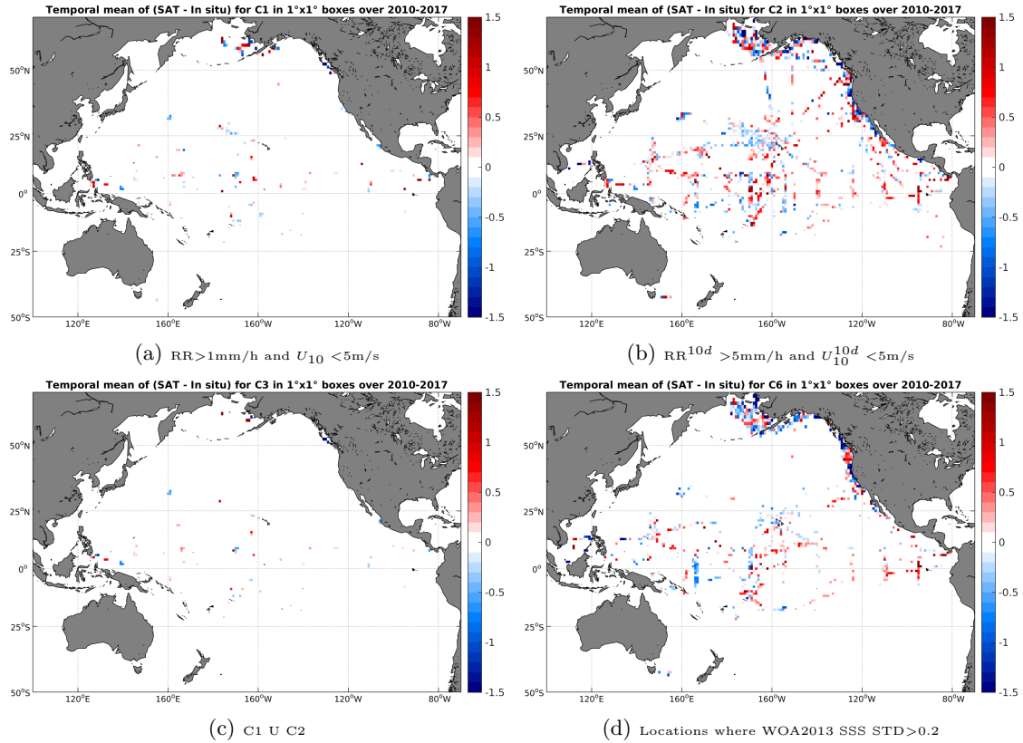
Figure 12: Temporal mean gridded over spatial boxes of size 1°x1° of \Delta SSS (SMOS-L3-CATDS-CECOS-IFREMER-V2-1DAY-0.5DEG - TSG-SAMOS) for 4 different subdatasets corresponding to: RR > 1mm/h and U_{10} < 5\text{m/s} (a), RR^{10d} > 5\text{mm/h} and U_{10}^{10d} < 5\text{m/s} (b), C1 U C2 (c), Locations where WOA2013 SSS STD > 0.2 (d).
