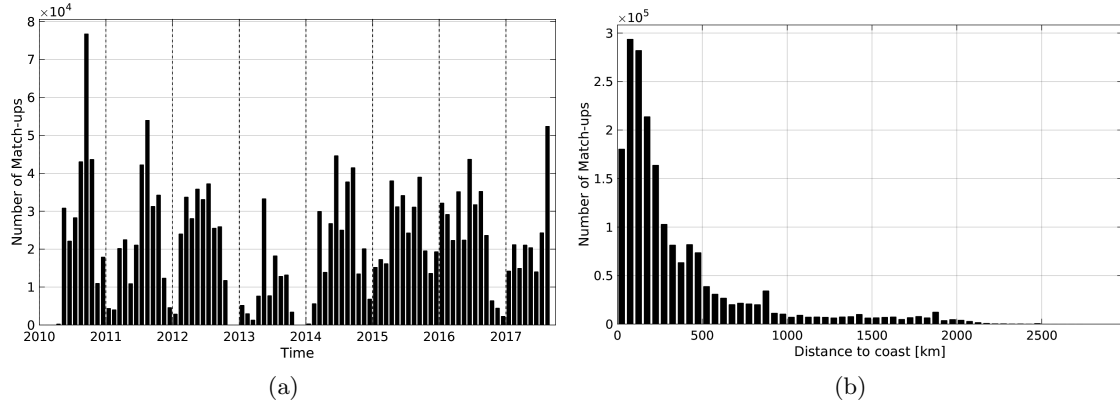
Figure 1: Number of match-ups between TSG-SAMOS and SMOS-L3-CATDS-CECOS-IFREMER-V2-1DAY-0.5DEG SSS as a function of time (a) and as function of the distance to coast (b) over the Pacific Ocean Pi-MEP region and for the full satellite product period.
