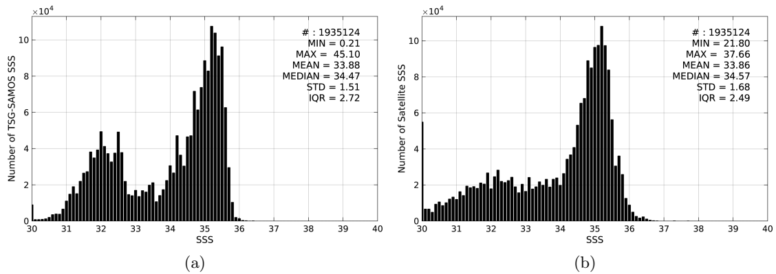
Figure 2: Histograms of SSS from TSG-SAMOS (a) and SMOS-L3-CATDS-CECOS-IFREMER-V2-1DAY-0.5DEG (b) considering all match-up pairs per bins of 0.1 over the Pacific Ocean Pi-MEP region and for the full satellite product period.
