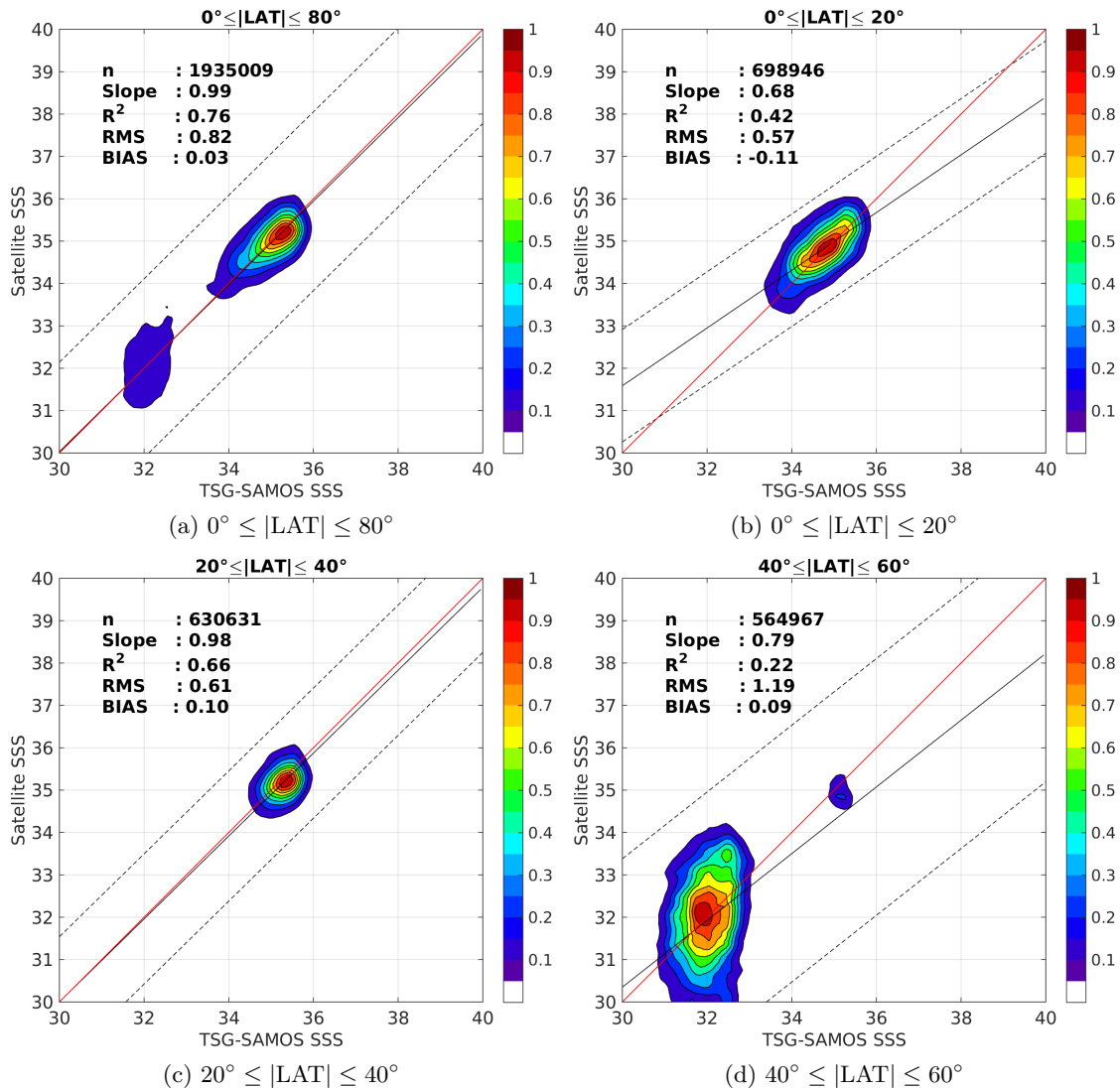
Figure 9: Contour maps of the concentration of SMOS-L3-CATDS-CECOS-IFREMER-V2-1DAY-0.5DEG SSS (y-axis) versus TSG-SAMOS SSS (x-axis) at match-up pairs for different latitude bands. For each plot, the red line shows x=y . The black thin and dashed lines indicate a linear fit through the data cloud and the \pm 95\% confidence levels, respectively. The number match-up pairs n , the slope and R^2 coefficient of the linear fit, the root mean square (RMS) and the mean bias between satellite and in situ data are indicated for each latitude band in each plots.
