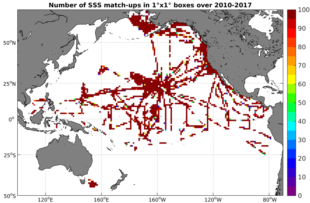
Figure 4: Number of SSS match-ups between TSG-SAMOS SSS and the SMOS-L3-CATDS-CECOS-IFREMER-V2-1DAY-0.5deg SSS product for the Pacific Ocean Pi-MEP region over 1°x1° boxes and for the full satellite product period.
