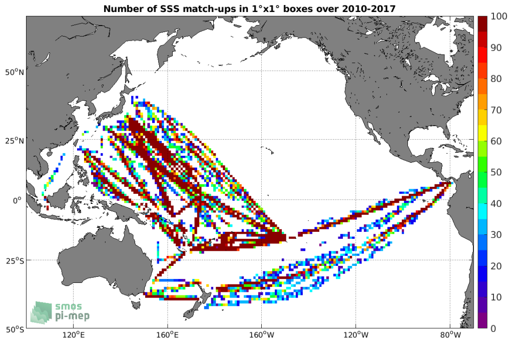
Figure 4: Number of SSS match-ups between TSG (LEGOS-DM) SSS and the SMOS SSS L3 v2 - Daily - 0.5 Deg (CATDS-CECOS-IFREMER) SSS product for the Pacific Ocean Pi-MEP region over 1^\circ \times 1^\circ boxes and for the full satellite product period.
