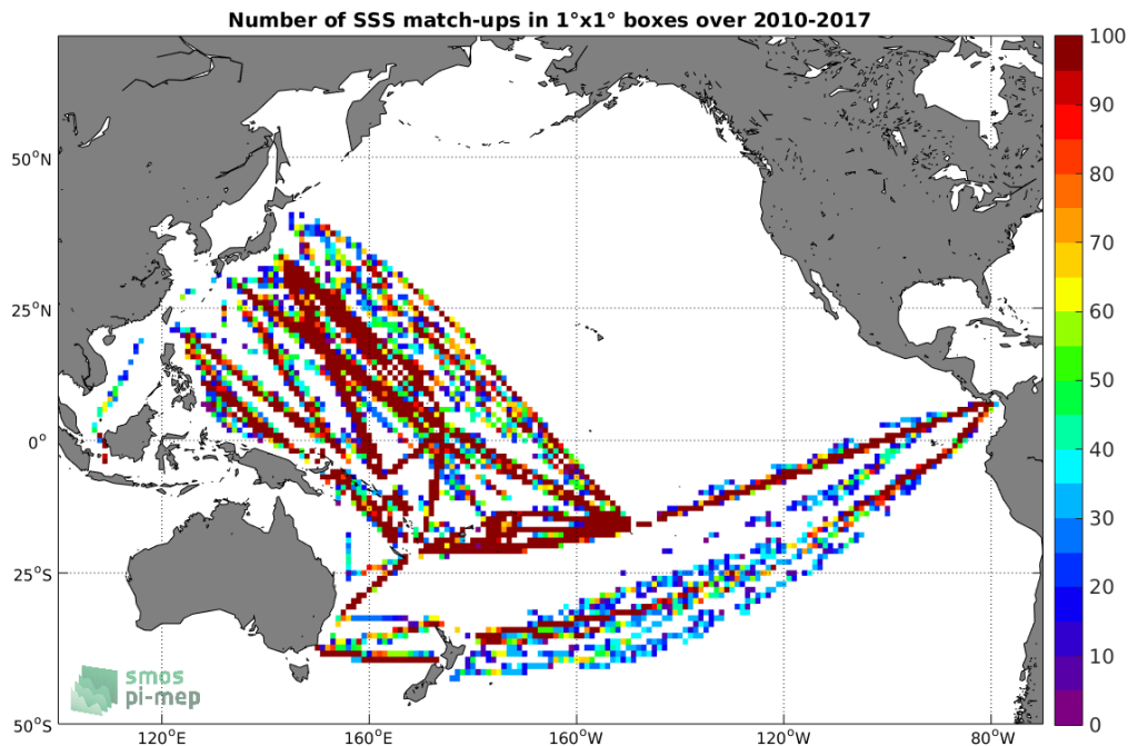
Figure 4: Number of SSS match-ups between TSG (LEGOS-DM) SSS and the SMOS SSS L3 v2 - Daily - 0.5 Deg (CATDS-CECOS-IFREMER) SSS product for the Pacific Ocean Pi-MEP region over 1°x1° boxes and for the full satellite product period.
