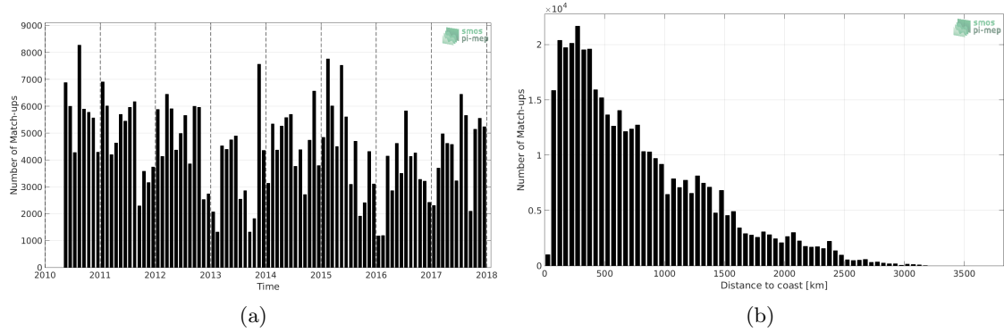
Figure 1: Number of match-ups between TSG (LEGOS-DM) and SMOS SSS L3 v2 - Daily - 0.5 Deg (CATDS-CECOS-IFREMER) SSS as a function of time (a) and as function of the distance to coast (b) over the Pacific Ocean Pi-MEP region and for the full satellite product period.
