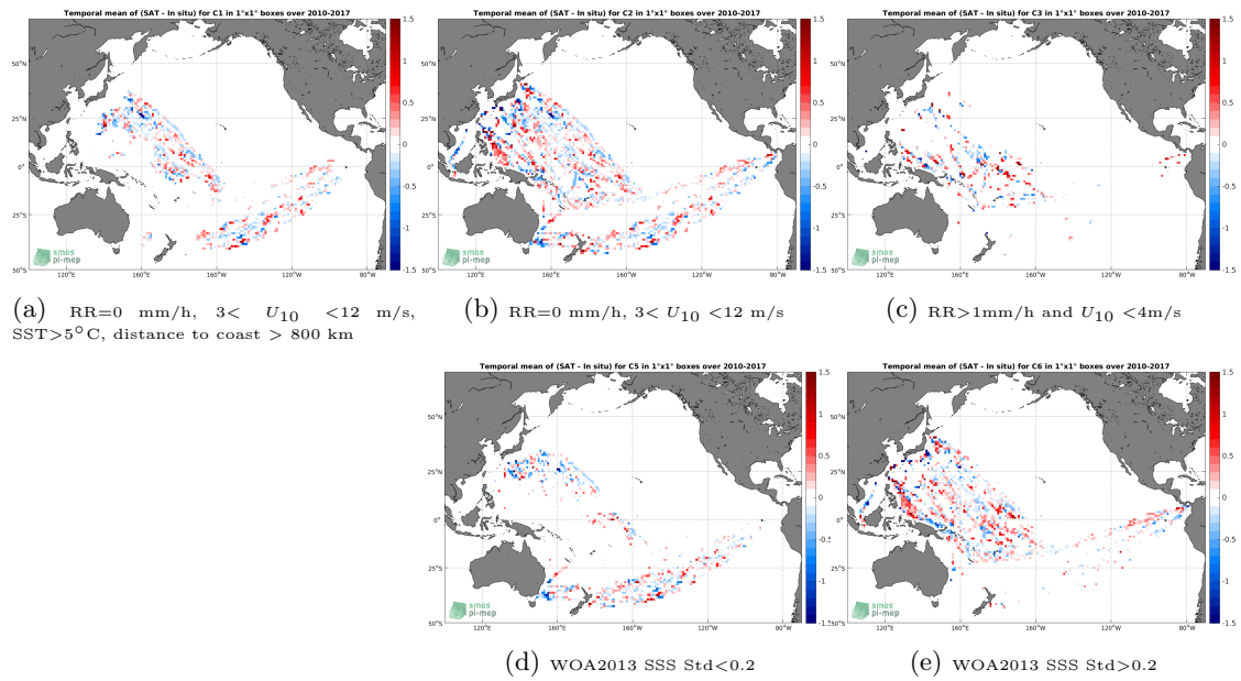
Figure 12: Temporal mean gridded over spatial boxes of size 1^\circ \times 1^\circ of \Delta SSS (SMOS SSS L3 v2 - Daily - 0.5 Deg (CATDS-CECOS-IFREMER) - TSG (LEGOS-DM)) for 5 different subdatasets corresponding to:RR=0 mm/h, 3 < U_{10} < 12 m/s, SST >5^\circ C, distance to coast > 800 km (a), RR=0 mm/h, 3 < U_{10} < 12 m/s (b), RR >1 mm/h and U_{10} < 4 m/s (c), WOA2013 SSS Std <0.2 (d), WOA2013 SSS Std >0.2 (e).
