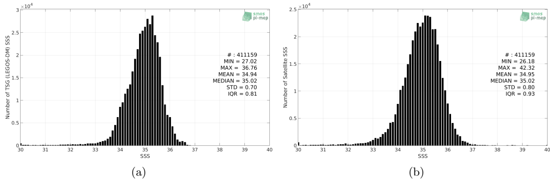
Figure 2: Histograms of SSS from TSG (LEGOS-DM) (a) and SMOS SSS L3 v2 - Daily - 0.5 Deg (CATDS-CECOS-IFREMER) (b) considering all match-up pairs per bins of 0.1 over the Pacific Ocean Pi-MEP region and for the full satellite product period.
