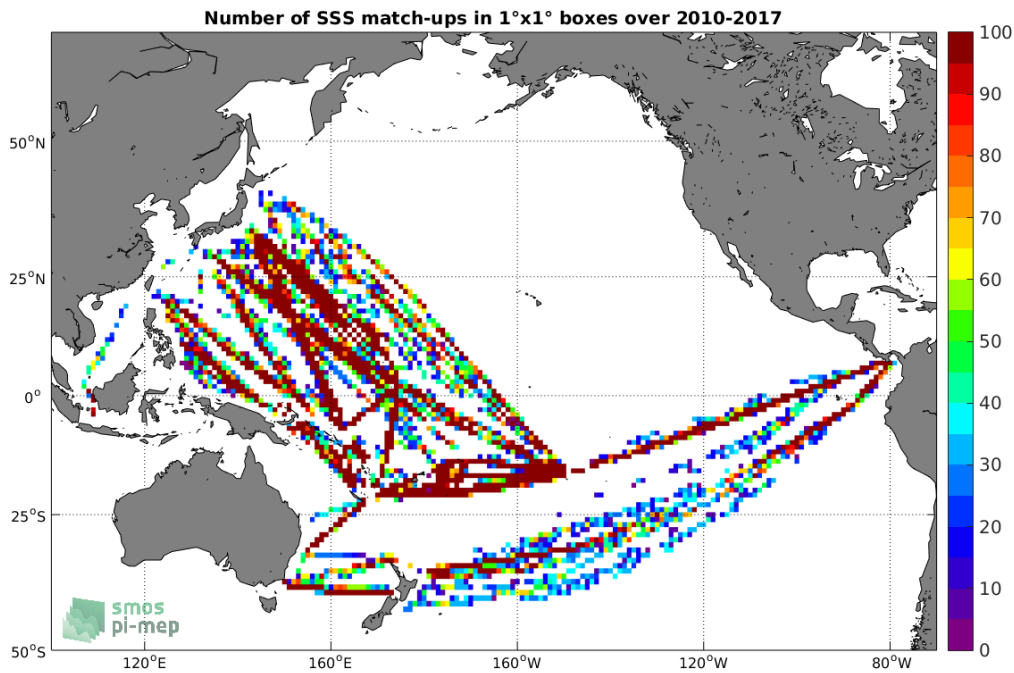
Figure 4: Number of SSS match-ups between TSG-LEGOS-DM SSS and the SMOS L3 v2 - Daily - 0.5 Deg (CATDS-CECOS-IFREMER) SSS product for the Pacific Ocean Pi-MEP region over 1^\circ \times 1^\circ boxes and for the full satellite product period.
