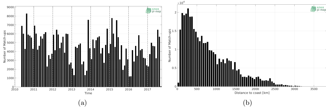
Figure 1: Number of match-ups between TSG-LEGOS-DM and SMOS L3 v2 - Daily - 0.5 Deg (CATDS-CECOS-IFREMER) SSS as a function of time (a) and as function of the distance to coast (b) over the Pacific Ocean Pi-MEP region and for the full satellite product period.
