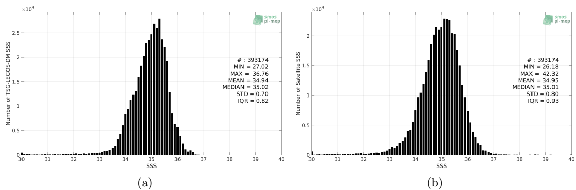
Figure 2: Histograms of SSS from TSG-LEGOS-DM (a) and SMOS L3 v2 - Daily - 0.5 Deg (CATDS-CECOS-IFREMER) (b) considering all match-up pairs per bins of 0.1 over the Pacific Ocean Pi-MEP region and for the full satellite product period.
