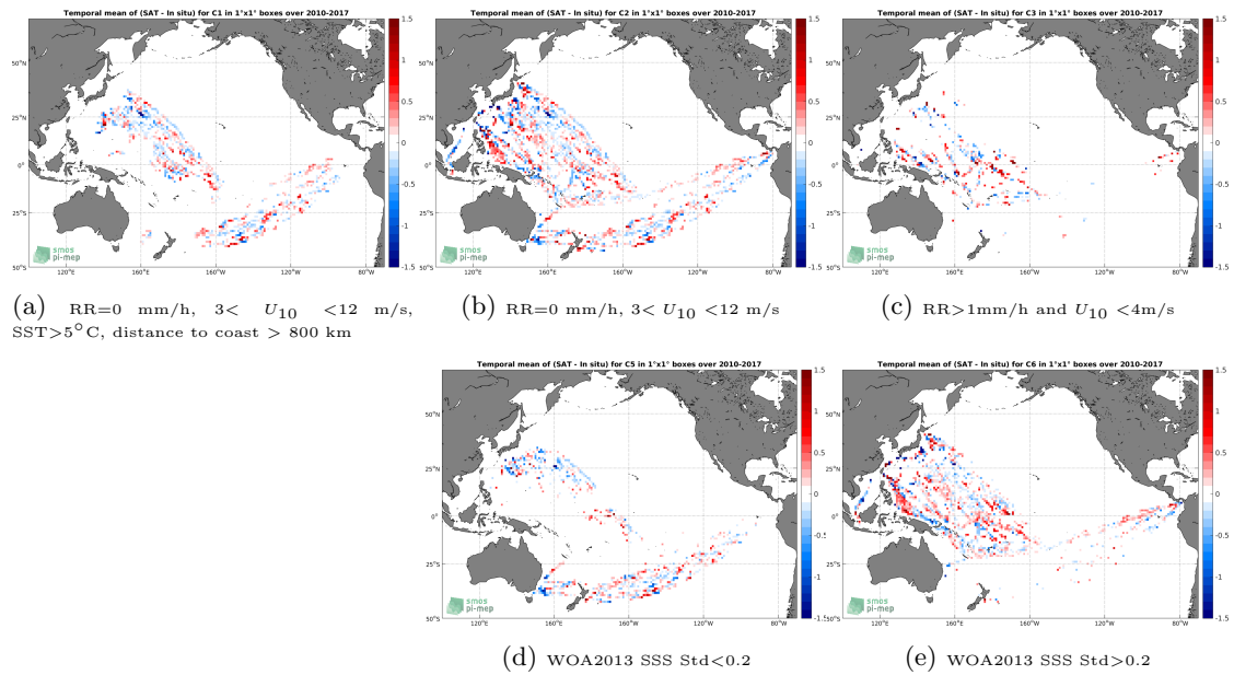
Figure 12: Temporal mean gridded over spatial boxes of size 1^\circ \times 1^\circ of \Delta SSS (SMOS L3 v2 - Daily - 0.5 Deg (CATDS-CECOS-IFREMER) - TSG-LEGOS-DM) for 5 different subdatasets corresponding to:RR=0 mm/h, 3 < U_{10} < 12 m/s, SST >5^\circ C, distance to coast > 800 km (a), RR=0 mm/h, 3 < U_{10} < 12 m/s (b), RR >1 mm/h and U_{10} < 4 m/s (c), WOA2013 SSS Std <0.2 (d), WOA2013 SSS Std >0.2 (e).
