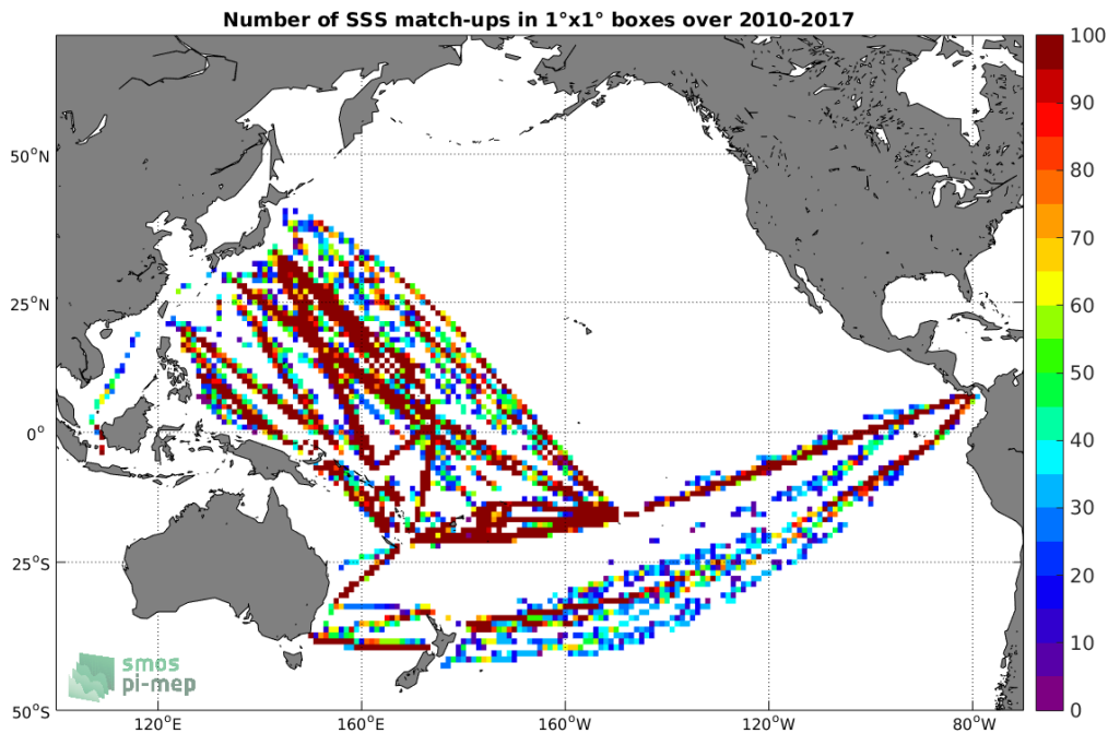
Figure 4: Number of SSS match-ups between TSG-LEGOS-DM SSS and the SMOS-L3-CATDS-CECOS-IFREMER-V2-1DAY-0.5DEG SSS product for the Pacific Ocean Pi-MEP region over 1°x1° boxes and for the full satellite product period.
