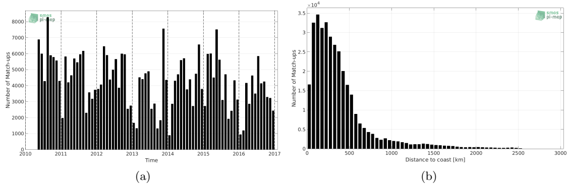
Figure 1: Number of match-ups between TSG-LEGOS-DM and SMOS-L3-CATDS-CECOS-IFREMER-V2-1DAY-0.5DEG SSS as a function of time (a) and as function of the distance to coast (b) over the Pacific Ocean Pi-MEP region and for the full satellite product period.
