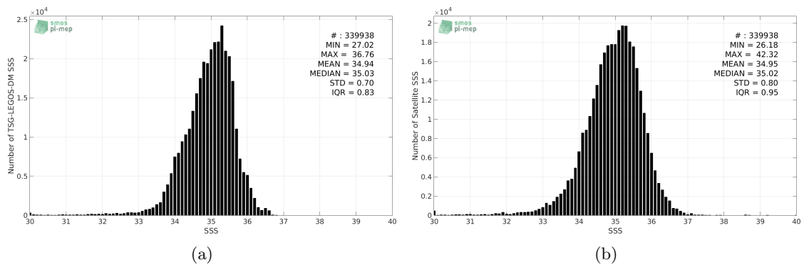
Figure 2: Histograms of SSS from TSG-LEGOS-DM (a) and SMOS-L3-CATDS-CECOS-IFREMER-V2-1DAY-0.5DEG (b) considering all match-up pairs per bins of 0.1 over the Pacific Ocean Pi-MEP region and for the full satellite product period.
