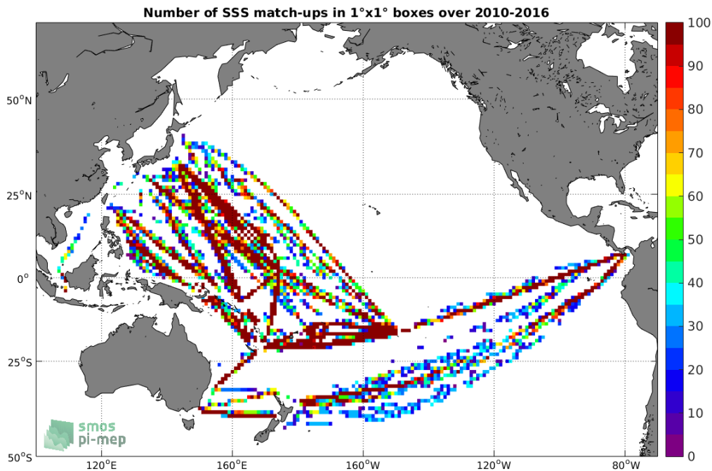
Figure 4: Number of SSS match-ups between TSG-LEGOS-DM SSS and the SMOS-L3-CATDS-CECOS-IFREMER-V2-1DAY-0.5DEG SSS product for the Pacific Ocean Pi-MEP region over 1^\circ \times 1^\circ boxes and for the full satellite product period.
