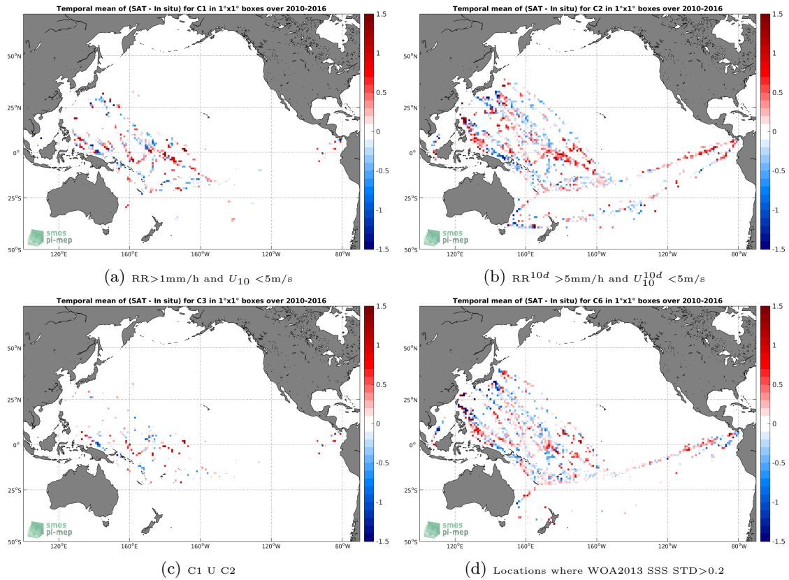
Figure 12: Temporal mean gridded over spatial boxes of size 1^\circ \times 1^\circ of \Delta SSS (SMOS-L3-CATDS-CECOS-IFREMER-V2-1DAY-0.5DEG - TSG-LEGOS-DM) for 4 different subdatasets corresponding to: RR > 1mm/h and U_{10} < 5\text{m/s} (a), RR^{10d} > 5\text{mm/h} and U_{10}^{10d} < 5\text{m/s} (b), C1 U C2 (c), Locations where WOA2013 SSS STD > 0.2 (d).
