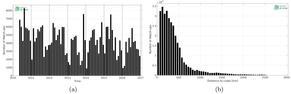
Figure 1: Number of match-ups between TSG-LEGOS-DM and SMOS-L3-CATDS-CECOS-IFREMER-V2-1DAY-0.5DEG SSS as a function of time (a) and as function of the distance to coast (b) over the Pacific Ocean Pi-MEP region and for the full satellite product period.
