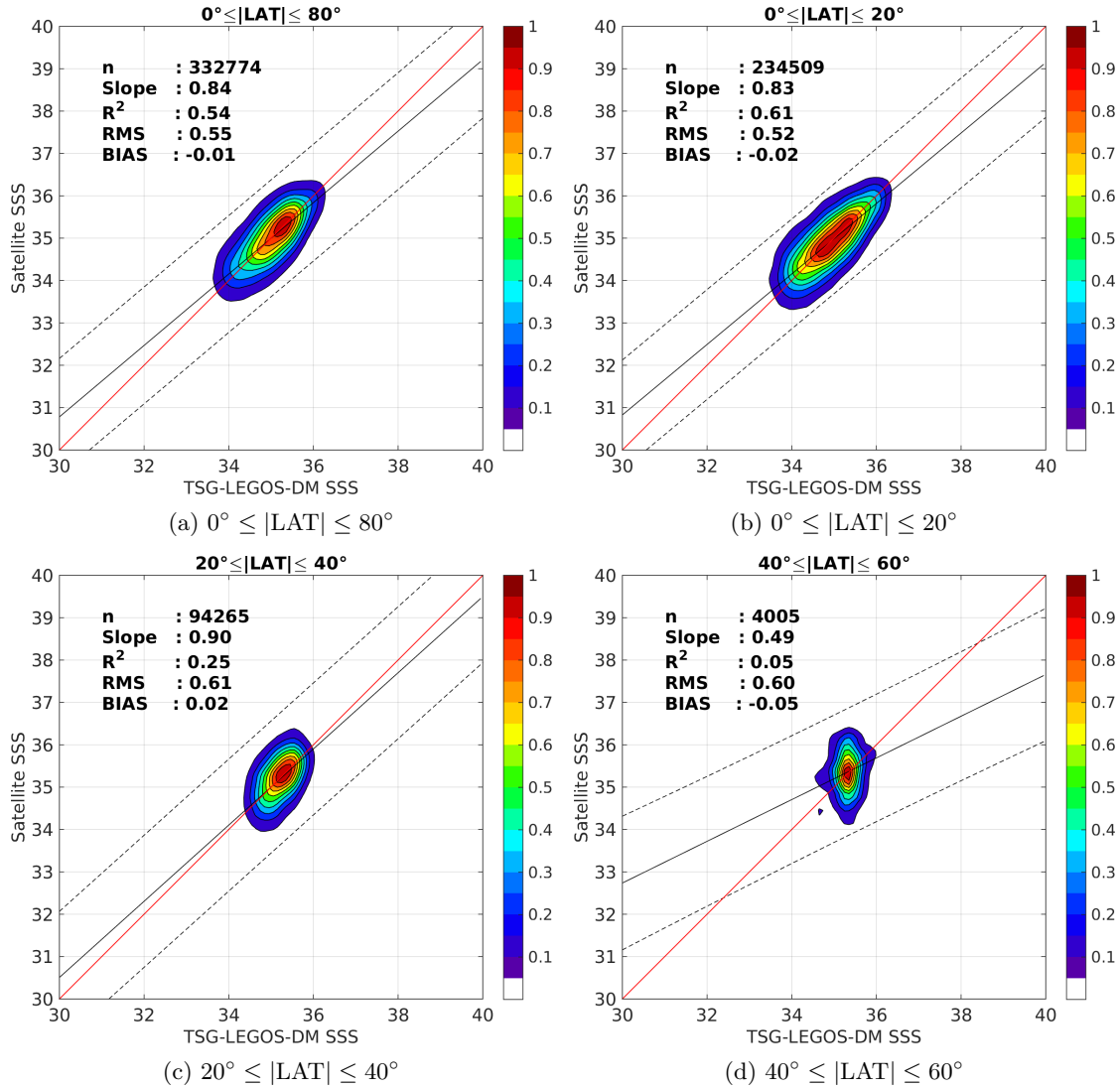
Figure 9: Contour maps of the concentration of SMOS-L3-CATDS-CECOS-IFREMER-V2-1DAY-0.5DEG SSS (y-axis) versus TSG-LEGOS-DM SSS (x-axis) at match-up pairs for different latitude bands. For each plot, the red line shows x=y . The black thin and dashed lines indicate a linear fit through the data cloud and the \pm 95\% confidence levels, respectively. The number match-up pairs n , the slope and R^2 coefficient of the linear fit, the root mean square (RMS) and the mean bias between satellite and in situ data are indicated for each latitude band in each plots.
