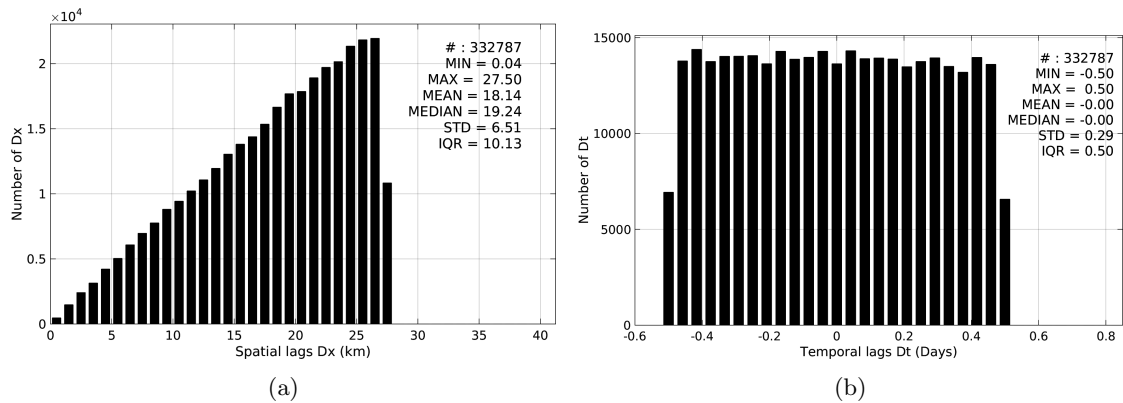
Figure 5: Histograms of the spatial (a) and temporal (b) lags between the time of the TSG-LEGOS-DM measurements and the date of the corresponding SMOS-L3-CATDS-CECOS-IFREMER-V2-1DAY-0.5DEG SSS product.
