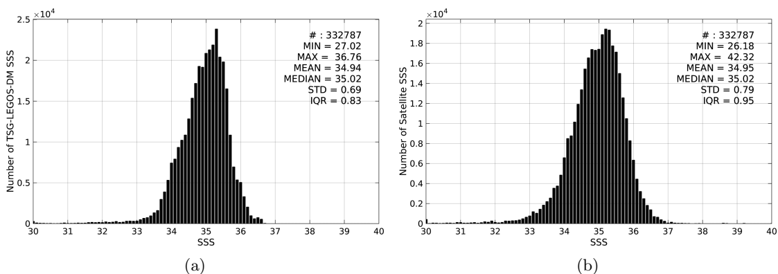
Figure 2: Histograms of SSS from TSG-LEGOS-DM (a) and SMOS-L3-CATDS-CECOS-IFREMER-V2-1DAY-0.5DEG (b) considering all match-up pairs per bins of 0.1 over the Pacific Ocean Pi-MEP region and for the full satellite product period.
