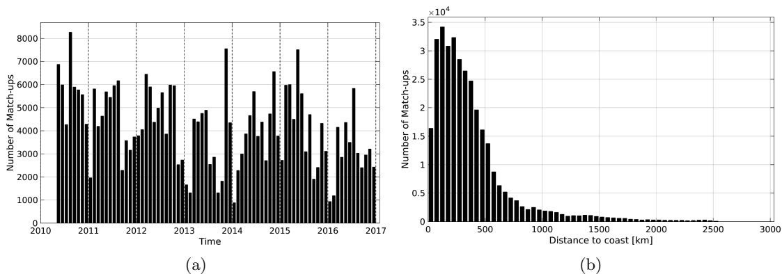
Figure 1: Number of match-ups between TSG-LEGOS-DM and SMOS-L3-CATDS-CECOS-IFREMER-V2-1DAY-0.5DEG SSS as a function of time (a) and as function of the distance to coast (b) over the Pacific Ocean Pi-MEP region and for the full satellite product period.
