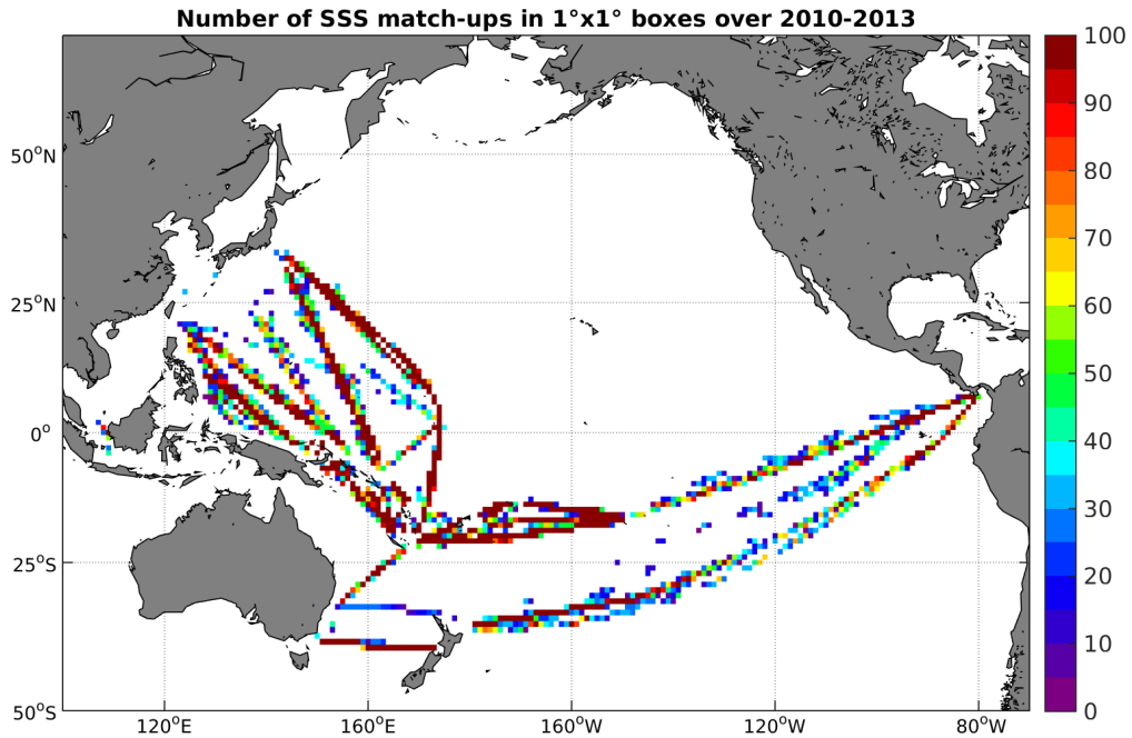
Figure 4: Number of SSS match-ups between TSG-LEGOS-DM SSS and the SMOS-L3-CATDS-CECOS-IFREMER-V2-1DAY-0.5deg SSS product for the Pacific Ocean Pi-MEP region over 1^\circ \times 1^\circ boxes and for the full satellite product period.
