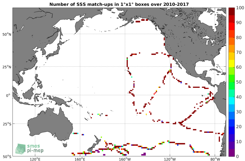
Figure 4: Number of SSS match-ups between TSG (GOSUD-Sailing-ship) SSS and the SMOS SSS L3 v2 - Daily - 0.5 Deg (CATDS-CECOS-IFREMER) SSS product for the Pacific Ocean Pi-MEP region over 1^\circ \times 1^\circ boxes and for the full satellite product period.
