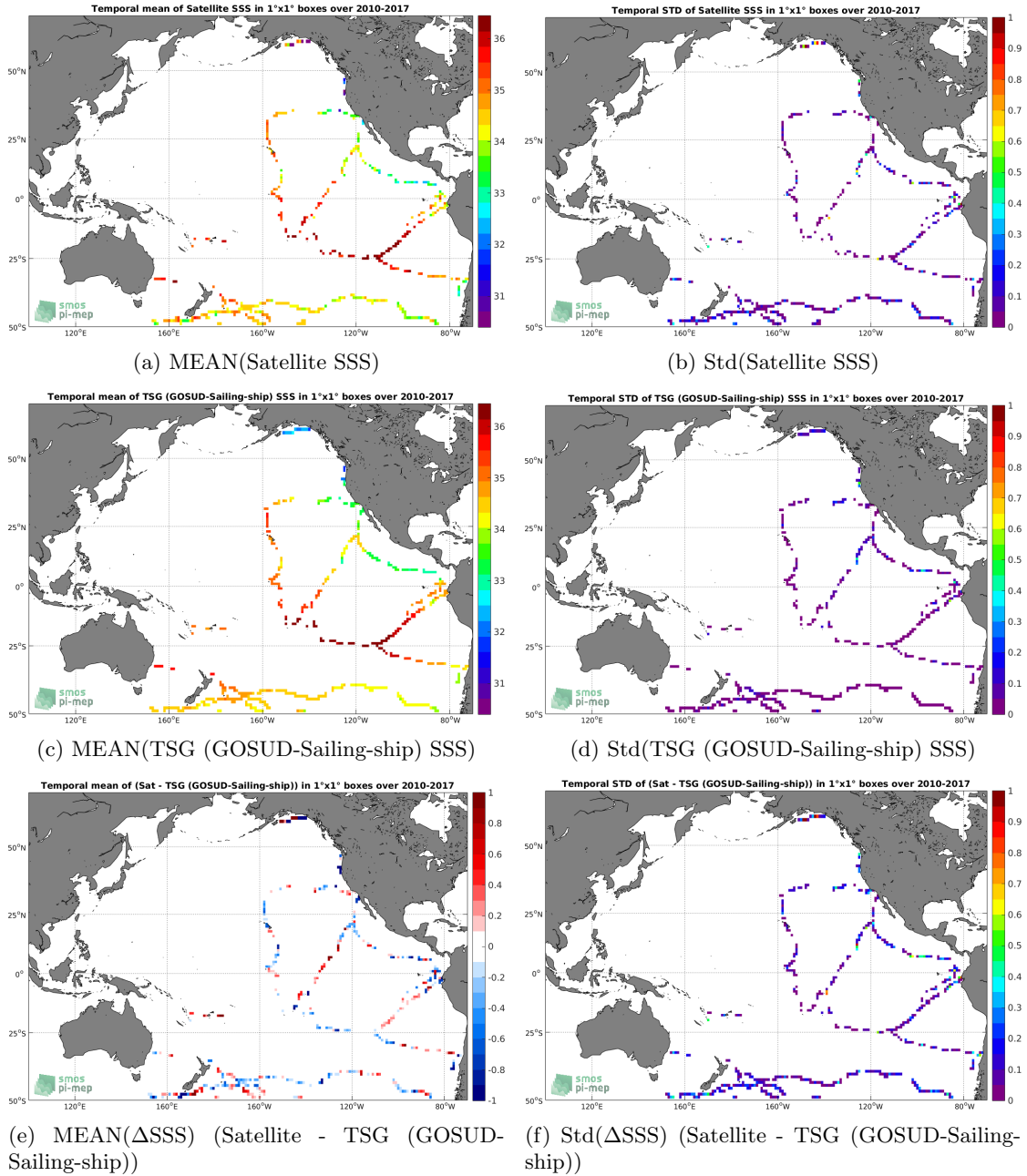
Figure 6: Temporal mean (left) and Std (right) of SSS from SMOS SSS L3 v2 - Daily - 0.5 Deg (CATDS-CECOS-IFREMER) (top), TSG (GOSUD-Sailing-ship) (middle), and of \Delta SSS (Satellite - TSG (GOSUD-Sailing-ship)). Only match-up pairs are used to generate these maps.
