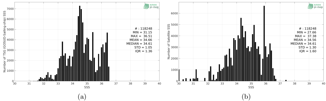
Figure 2: Histograms of SSS from TSG (GOSUD-Sailing-ship) (a) and SMOS SSS L3 v2 - Daily - 0.5 Deg (CATDS-CECOS-IFREMER) (b) considering all match-up pairs per bins of 0.1 over the Pacific Ocean Pi-MEP region and for the full satellite product period.
