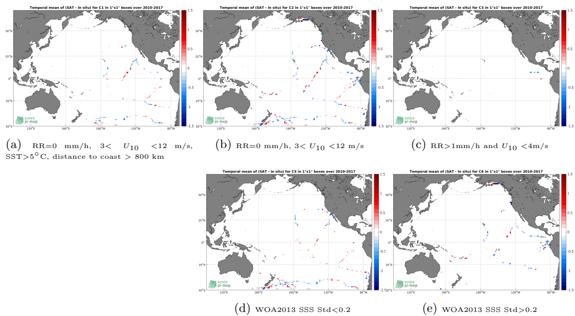
Figure 12: Temporal mean gridded over spatial boxes of size 1^\circ \times 1^\circ of \Delta SSS (SMOS L3 v2 - Daily - 0.5 Deg (CATDS-CECOS-IFREMER) - TSG-GOSUD-Sailing-ship) for 5 different subdatasets corresponding to:RR=0 mm/h, 3 < U_{10} < 12 m/s, SST > 5^\circ\text{C} , distance to coast > 800 km (a), RR=0 mm/h, 3 < U_{10} < 12 m/s (b), RR > 1 mm/h and U_{10} < 4 m/s (c), WOA2013 SSS Std < 0.2 (d), WOA2013 SSS Std > 0.2 (e).
