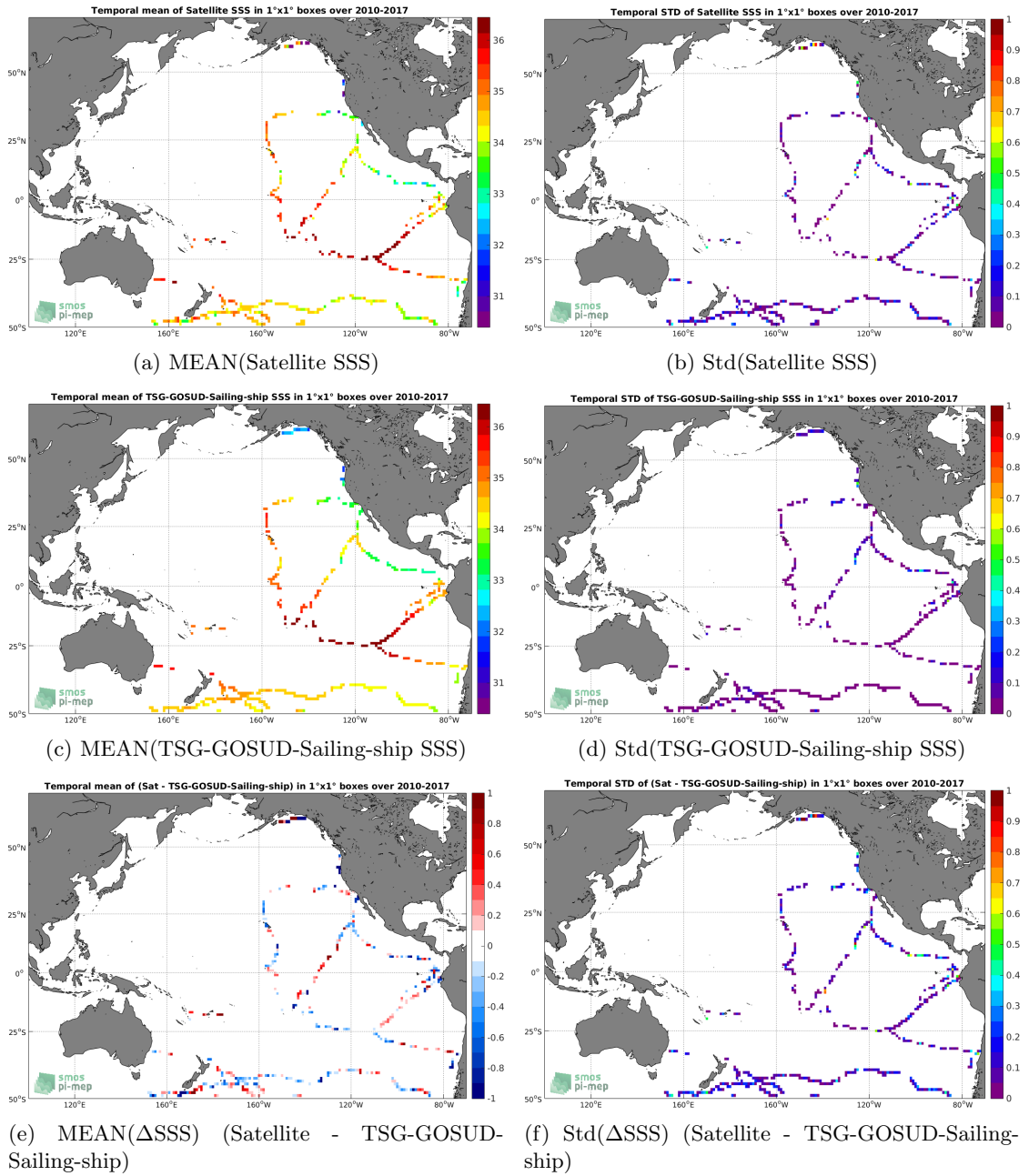
Figure 6: Temporal mean (left) and Std (right) of SSS from SMOS L3 v2 - Daily - 0.5 Deg (CATDS-CECOS-IFREMER) (top), TSG-GOSUD-Sailing-ship (middle), and of \Delta SSS (Satellite - TSG-GOSUD-Sailing-ship). Only match-up pairs are used to generate these maps.
