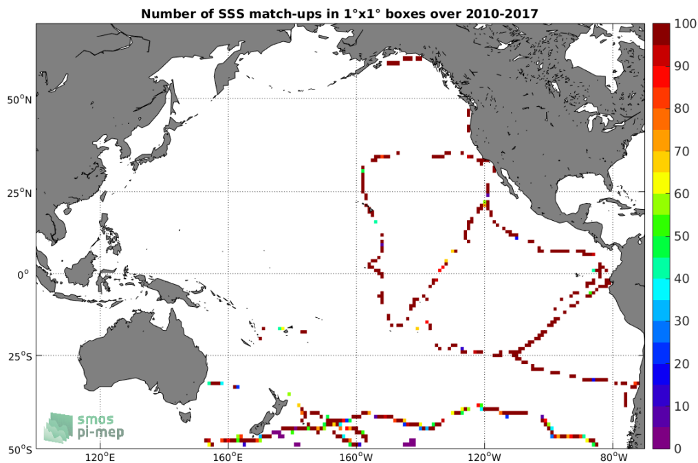
Figure 4: Number of SSS match-ups between TSG-GOSUD-Sailing-ship SSS and the SMOS L3 v2 - Daily - 0.5 Deg (CATDS-CECOS-IFREMER) SSS product for the Pacific Ocean Pi-MEP region over 1^\circ \times 1^\circ boxes and for the full satellite product period.
