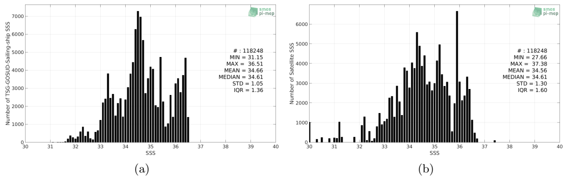
Figure 2: Histograms of SSS from TSG-GOSUD-Sailing-ship (a) and SMOS L3 v2 - Daily - 0.5 Deg (CATDS-CECOS-IFREMER) (b) considering all match-up pairs per bins of 0.1 over the Pacific Ocean Pi-MEP region and for the full satellite product period.
