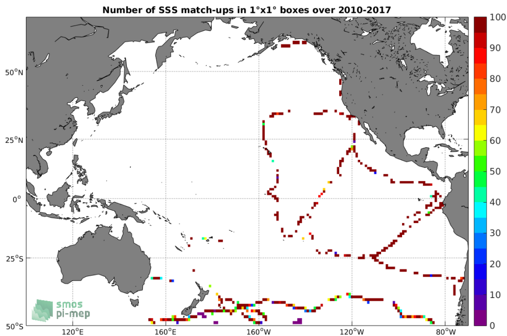
Figure 4: Number of SSS match-ups between TSG-GOSUD-Sailing-ship SSS and the SMOS-L3-CATDS-CECOS-IFREMER-V2-1DAY-0.5DEG SSS product for the Pacific Ocean Pi-MEP region over 1^\circ \times 1^\circ boxes and for the full satellite product period.
