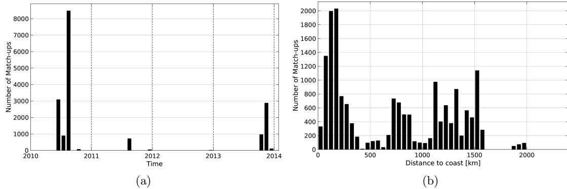
Figure 1: Number of match-ups between TSG-GOSUD-Sailing-ship and SMOS-L3-CATDS-CECOS-IFREMER-V2-1DAY-0.5DEG SSS as a function of time (a) and as function of the distance to coast (b) over the Pacific Ocean Pi-MEP region and for the full satellite product period.
