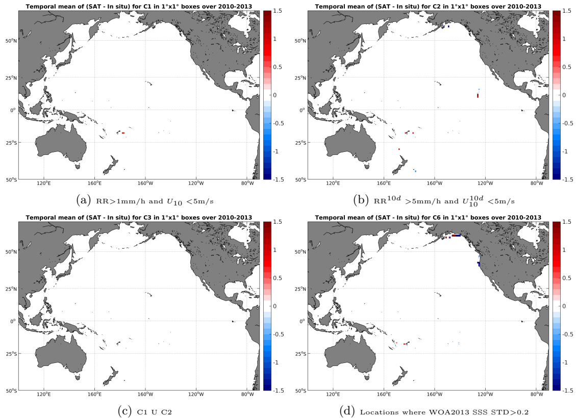
Figure 12: Temporal mean gridded over spatial boxes of size 1°x1° of \Delta SSS (SMOS-L3-CATDS-CECOS-IFREMER-V2-1DAY-0.5DEG - TSG-GOSUD-Sailing-ship) for 4 different subdatasets corresponding to:RR>1mm/h and U_{10} < 5\text{m/s} (a), RR^{10d} > 5\text{mm/h} and U_{10}^{10d} < 5\text{m/s} (b), C1 U C2 (c),Locations where WOA2013 SSS STD>0.2 (d).
