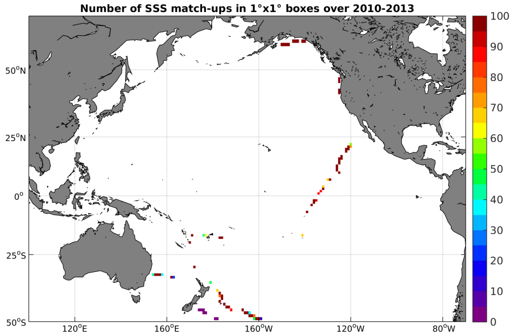
Figure 4: Number of SSS match-ups between TSG-GOSUD-Sailing-ship SSS and the SMOS-L3-CATDS-CECOS-IFREMER-V2-1DAY-0.5deg SSS product for the Pacific Ocean Pi-MEP region over 1°x1° boxes and for the full satellite product period.
