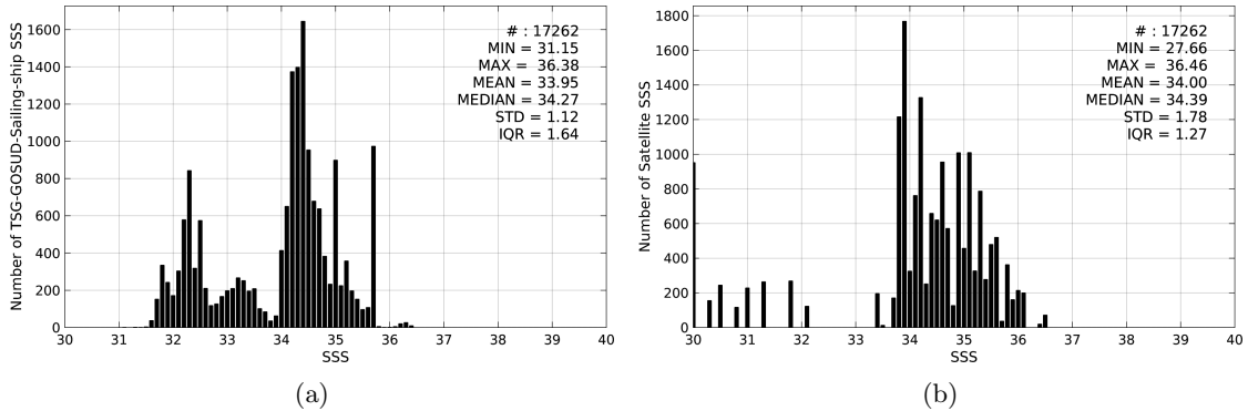
Figure 2: Histograms of SSS from TSG-GOSUD-Sailing-ship (a) and SMOS-L3-CATDS-CECOS-IFREMER-V2-1DAY-0.5deg (b) considering all match-up pairs per bins of 0.1 over the Pacific Ocean Pi-MEP region and for the full satellite product period.
