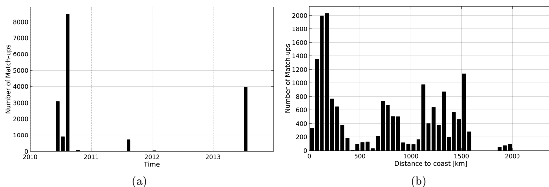
Figure 1: Number of match-ups between TSG-GOSUD-Sailing-ship and SMOS-L3-CATDS-CECOS-IFREMER-V2-1DAY-0.5deg SSS as a function of time (a) and as function of the distance to coast (b) over the Pacific Ocean Pi-MEP region and for the full satellite product period.
