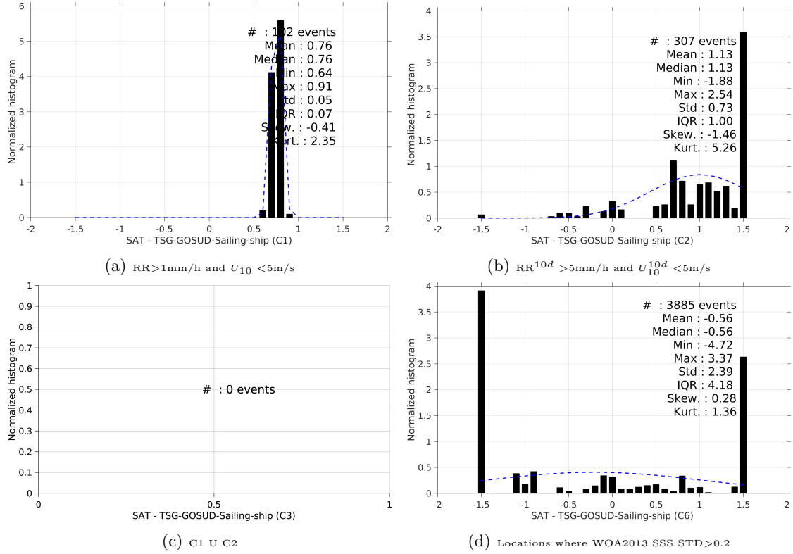
Figure 13: Normalized histogram of \Delta\text{SSS} (SMOS-L3-CATDS-CECOS-IFREMER-V2-1DAY-0.5deg - TSG-GOSUD-Sailing-ship) for 6 different subdatasets corresponding to: RR > 1mm/h and U_{10} < 5\text{m/s} (a), RR^{10d} > 5\text{mm/h} and U_{10}^{10d} < 5\text{m/s} (b), C1 U C2 (c), Locations where WOA2013 SSS STD > 0.2 (d).
