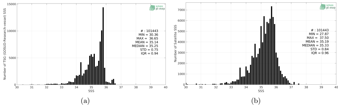
Figure 2: Histograms of SSS from TSG (GOSUD-Research-vessel) (a) and SMOS SSS L3 v2 - Daily - 0.5 Deg (CATDS-CECOS-IFREMER) (b) considering all match-up pairs per bins of 0.1 over the Pacific Ocean Pi-MEP region and for the full satellite product period.
