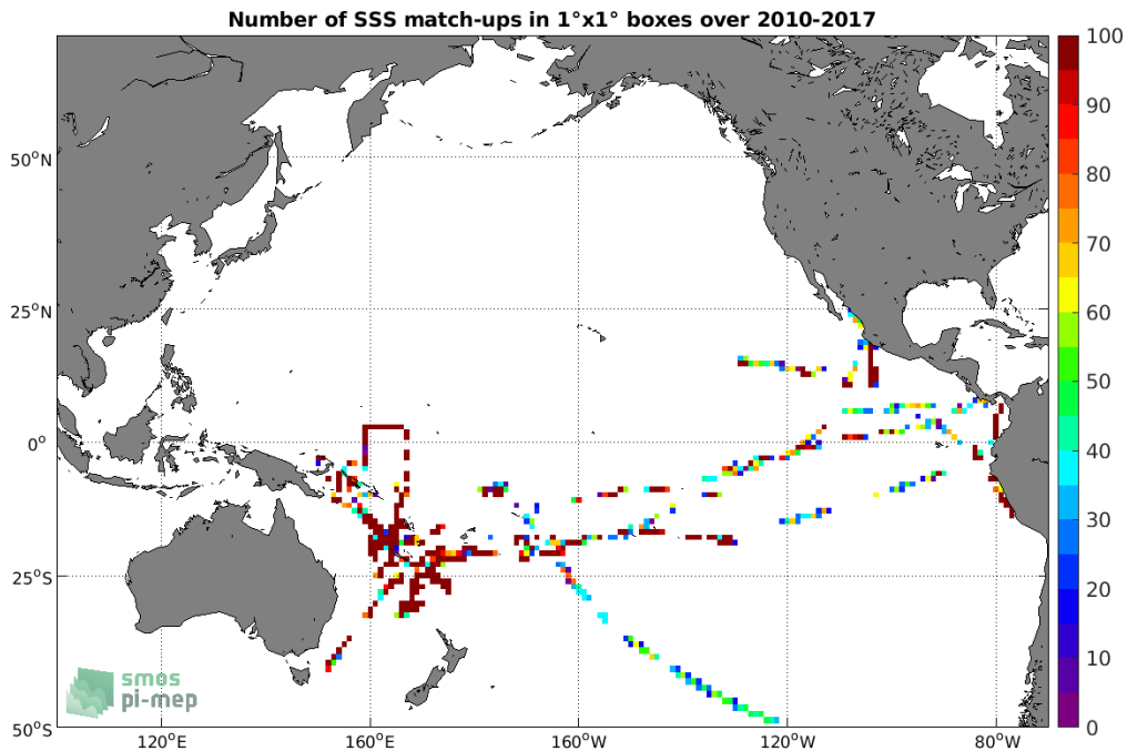
Figure 4: Number of SSS match-ups between TSG (GOSUD-Research-vessel) SSS and the SMOS SSS L3 v2 - Daily - 0.5 Deg (CATDS-CECOS-IFREMER) SSS product for the Pacific Ocean Pi-MEP region over 1°x1° boxes and for the full satellite product period.
