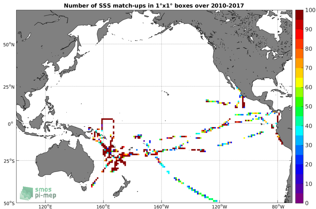
Figure 4: Number of SSS match-ups between TSG (GOSUD-Research-vessel) SSS and the SMOS SSS L3 v2 - Daily - 0.5 Deg (CATDS-CECOS-IFREMER) SSS product for the Pacific Ocean Pi-MEP region over 1^\circ \times 1^\circ boxes and for the full satellite product period.
