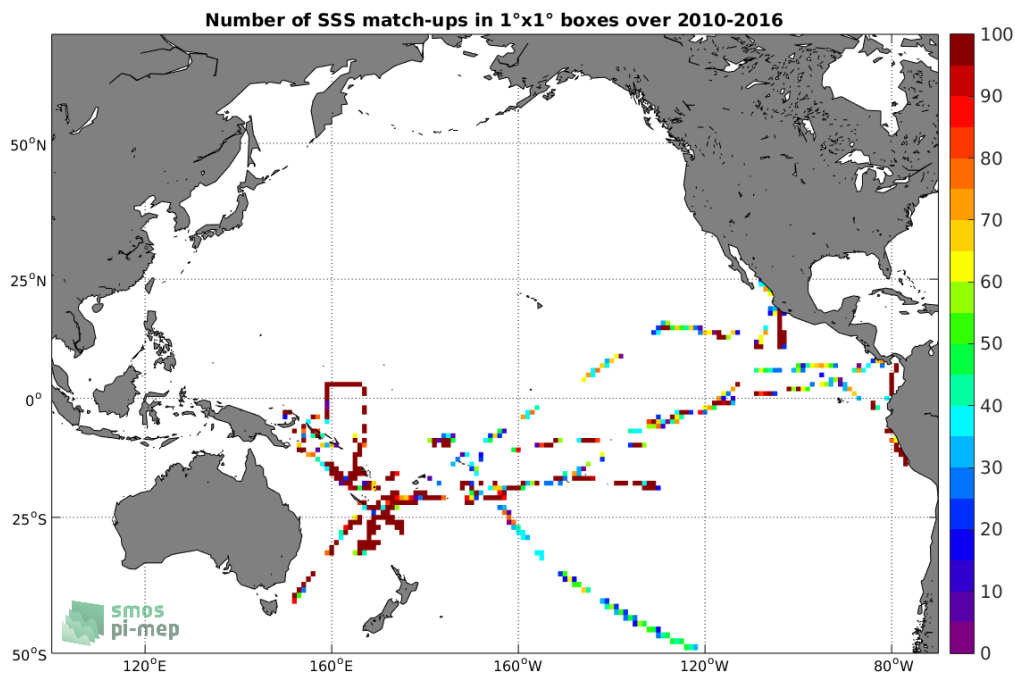
Figure 4: Number of SSS match-ups between TSG-GOSUD-Research-vessel SSS and the SMOS-L3-CATDS-CECOS-IFREMER-V2-1DAY-0.5DEG SSS product for the Pacific Ocean Pi-MEP region over 1^\circ \times 1^\circ boxes and for the full satellite product period.
