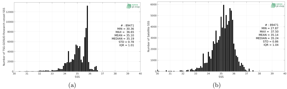
Figure 2: Histograms of SSS from TSG-GOSUD-Research-vessel (a) and SMOS-L3-CATDS-CECOS-IFREMER-V2-1DAY-0.5DEG (b) considering all match-up pairs per bins of 0.1 over the Pacific Ocean Pi-MEP region and for the full satellite product period.
