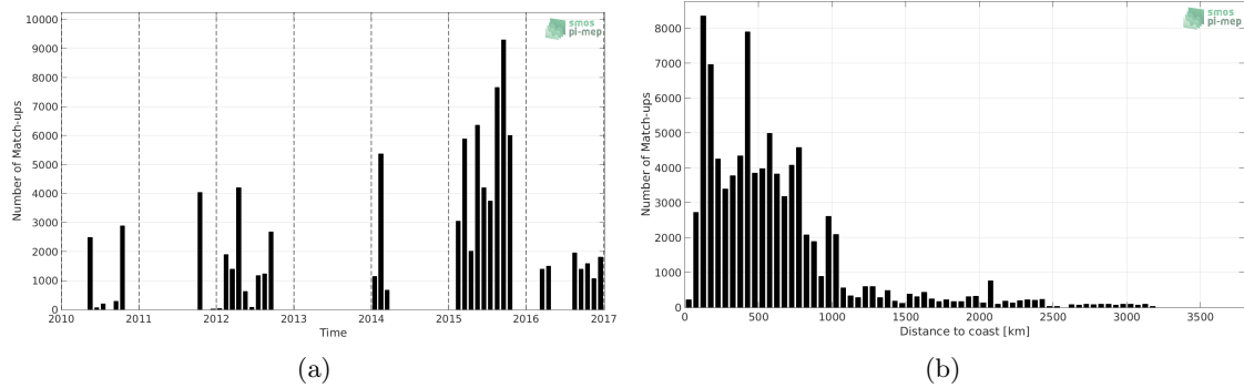
Figure 1: Number of match-ups between TSG-GOSUD-Research-vessel and SMOS-L3-CATDS-CECOS-IFREMER-V2-1DAY-0.5DEG SSS as a function of time (a) and as function of the distance to coast (b) over the Pacific Ocean Pi-MEP region and for the full satellite product period.
