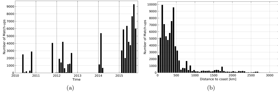
Figure 1: Number of match-ups between TSG-GOSUD-Research-vessel and SMOS-L3-CATDS-CECOS-IFREMER-V2-1DAY-0.5DEG SSS as a function of time (a) and as function of the distance to coast (b) over the Pacific Ocean Pi-MEP region and for the full satellite product period.
