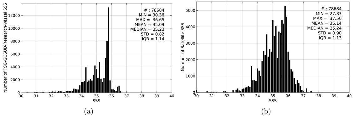
Figure 2: Histograms of SSS from TSG-GOSUD-Research-vessel (a) and SMOS-L3-CATDS-CECOS-IFREMER-V2-1DAY-0.5DEG (b) considering all match-up pairs per bins of 0.1 over the Pacific Ocean Pi-MEP region and for the full satellite product period.
