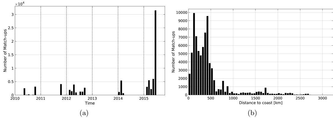
Figure 1: Number of match-ups between TSG-GOSUD-Research-vessel and SMOS-L3-CATDS-CECOS-IFREMER-V2-1DAY-0.5deg SSS as a function of time (a) and as function of the distance to coast (b) over the Pacific Ocean Pi-MEP region and for the full satellite product period.
