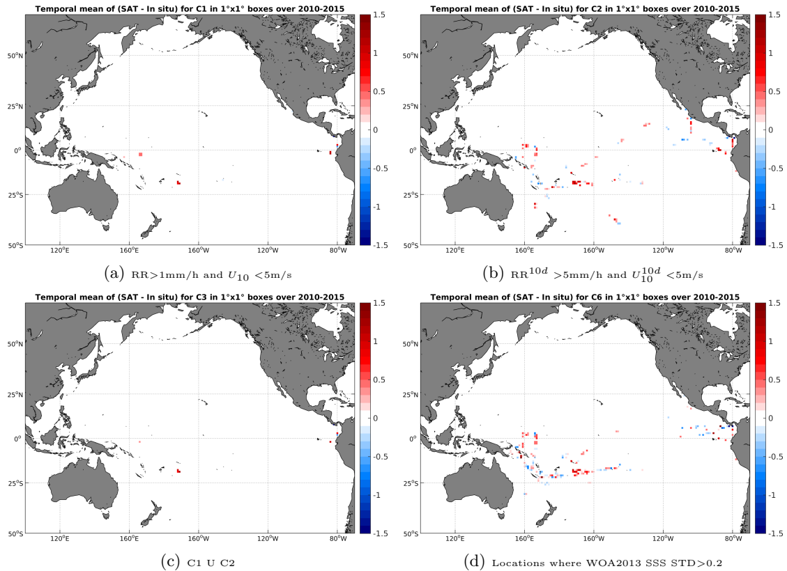
Figure 12: Temporal mean gridded over spatial boxes of size 1°x1° of \Delta SSS (SMOS-L3-CATDS-CECOS-IFREMER-V2-1DAY-0.5deg - TSG-GOSUD-Research-vessel) for 4 different subdatasets corresponding to:RR>1mm/h and U_{10} < 5m/s (a), RR^{10d} > 5mm/h and U_{10}^{10d} < 5m/s (b), C1 U C2 (c),Locations where WOA2013 SSS STD>0.2 (d).
